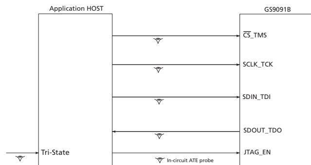
Figure 3-22: System JTAG
