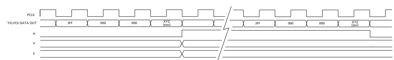
Figure 3-15: H,V,F Timing In Low-latency Mode
