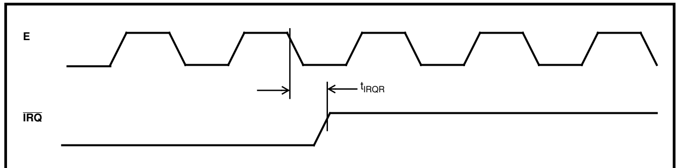
Figure 19 - Interrupt Request Release Time
