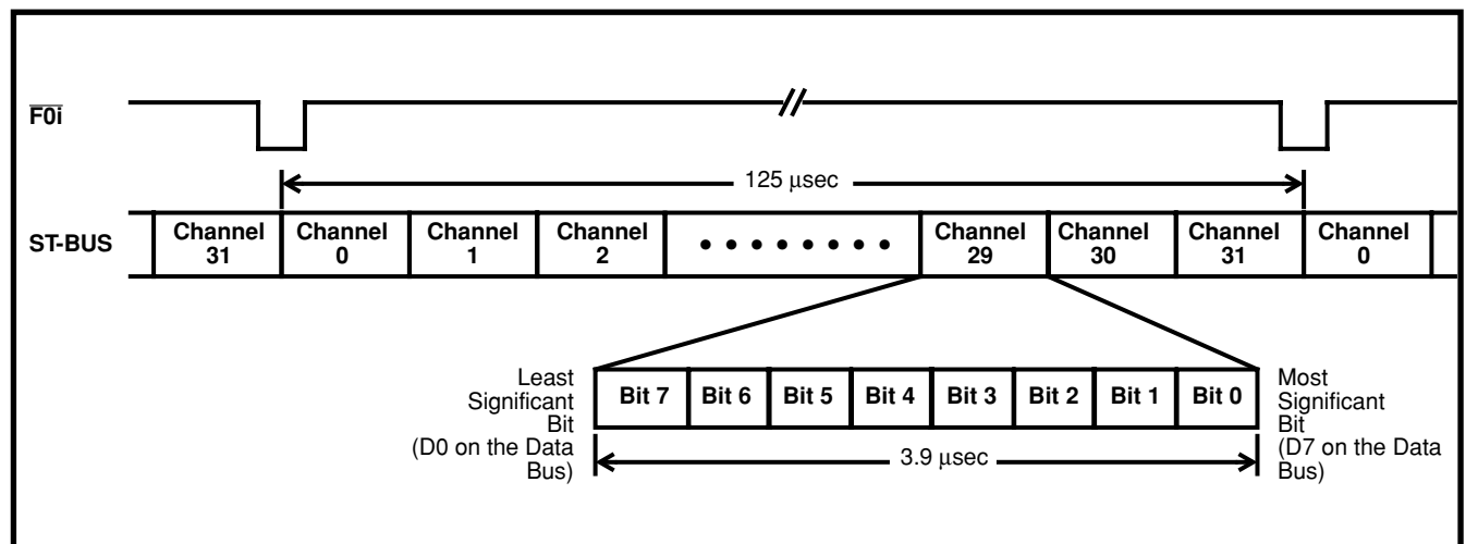
Figure 24 - ST-BUS Format
