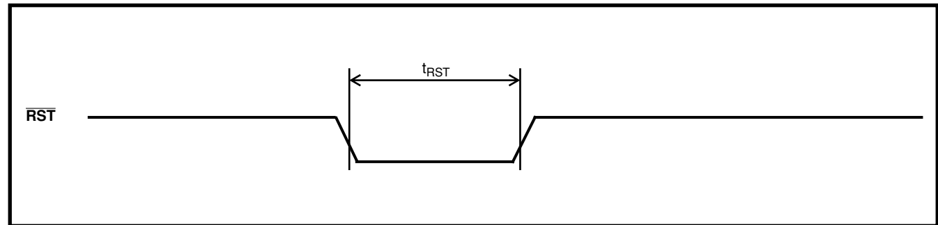
Figure 21 - RESET Timing
