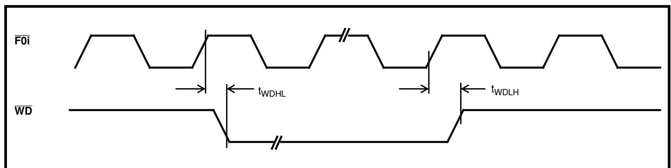
Figure 20 - Watchdog Timer Input and Output
