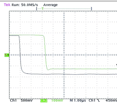
Figure 39. Turn-Off Response
