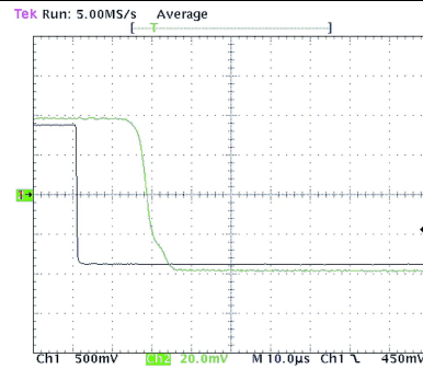
Figure 37. Turn-Off Response
