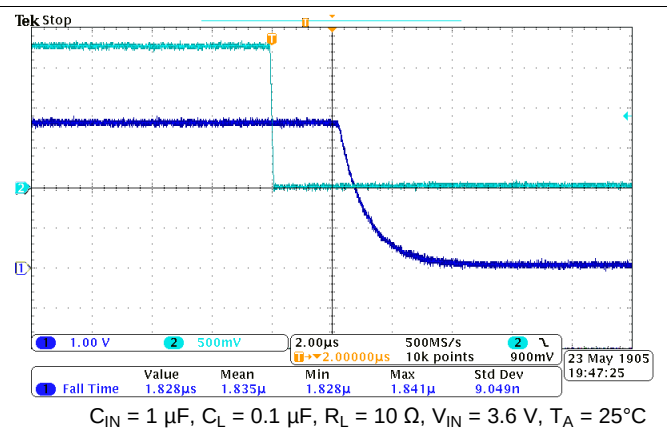
Figure 21. Turn-Off Response
