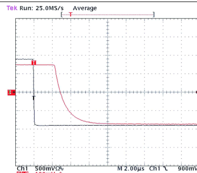
Figure 37. Turn-Off Response
