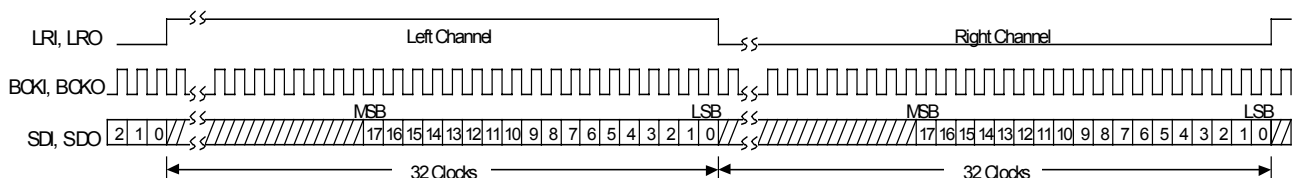
Fig. 3-9 Right-Justified Data Format 64Fs, 18bit Data
