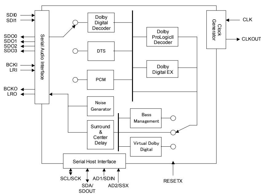
Fig.1-2 NJU26501 Function Diagram
