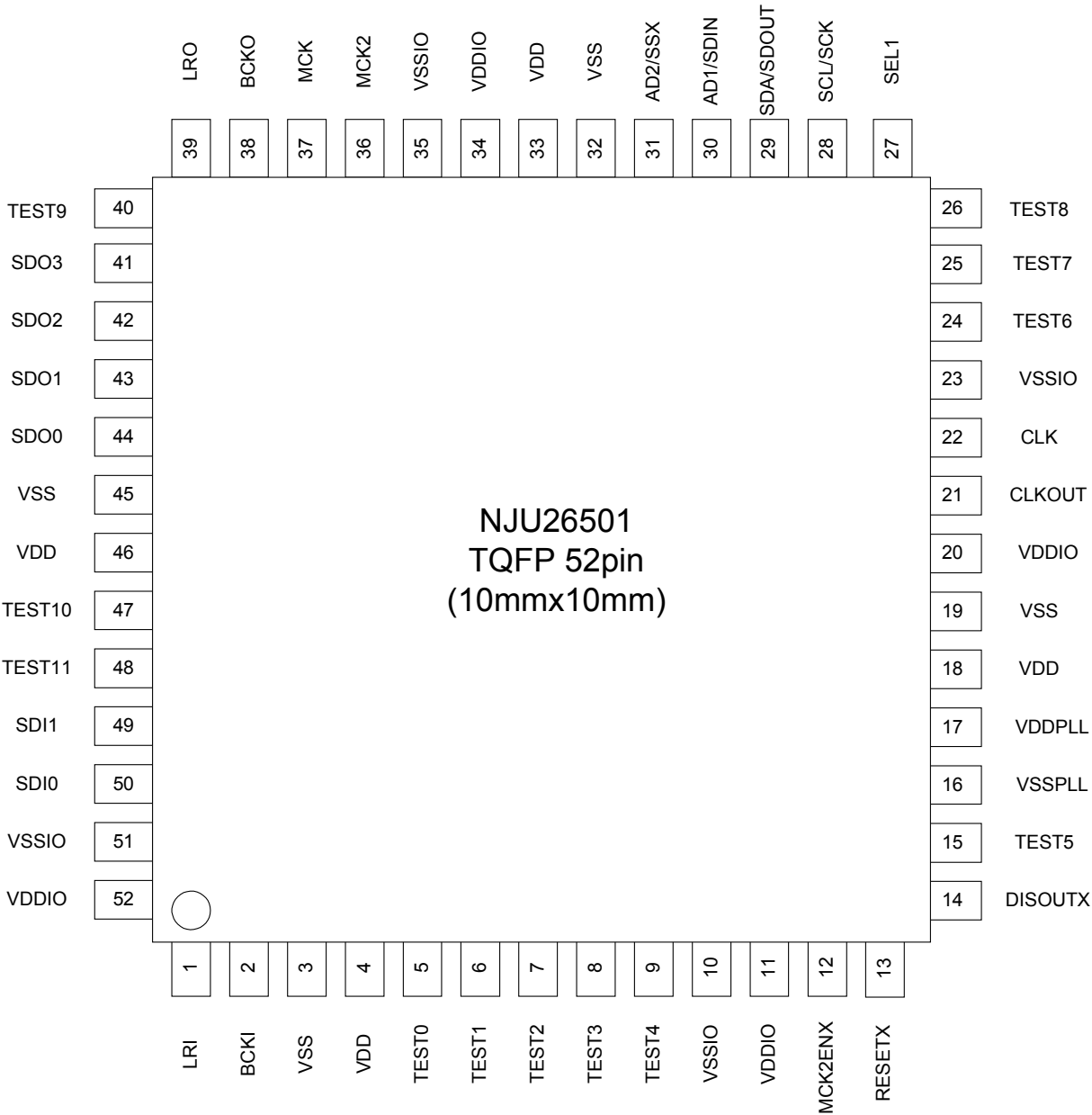
Fig.1-3 Pin Configuration
