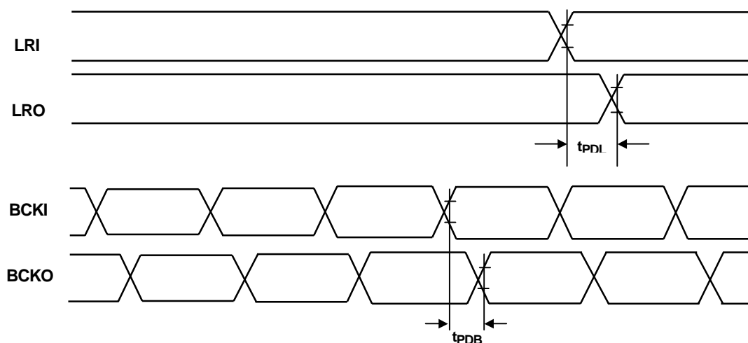
Fig. 3-16 Serial Audio Clock Timing (SLAVE mode)
