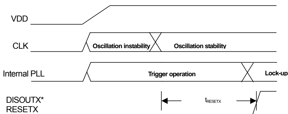
Fig. 1-7 Reset Timing
