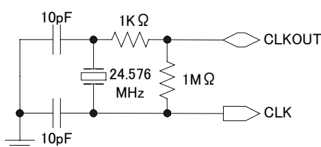
Fig.1-6 The example of the oscillator circuit.
