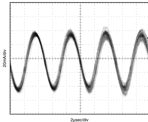
Input Reflected Ripple Current
