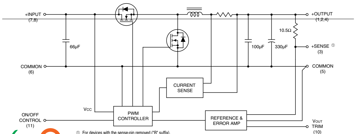
Figure 1. Simplified Schematic
