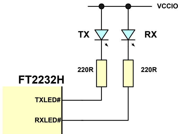
Figure 4.19 Dual LED UART Configuration
