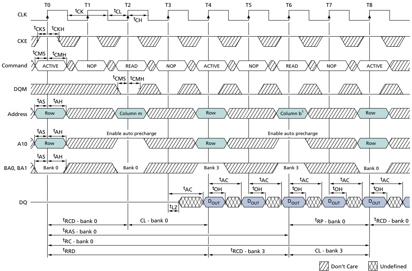
Figure 21: Alternating Bank Read Accesses
