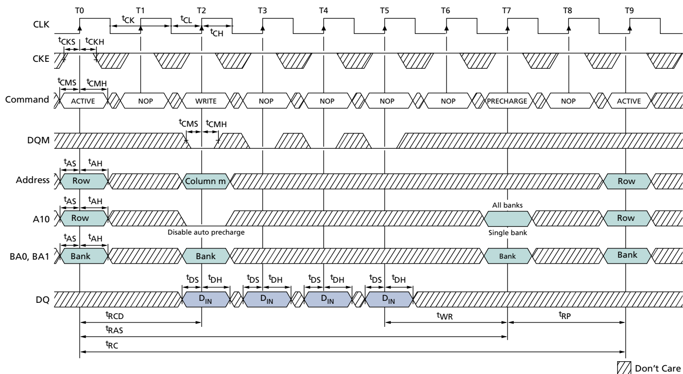
Figure 42: WRITE Without Auto Precharge
