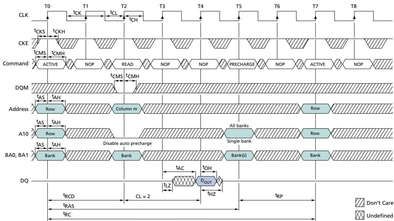
Figure 38: Single READ Without Auto Precharge
