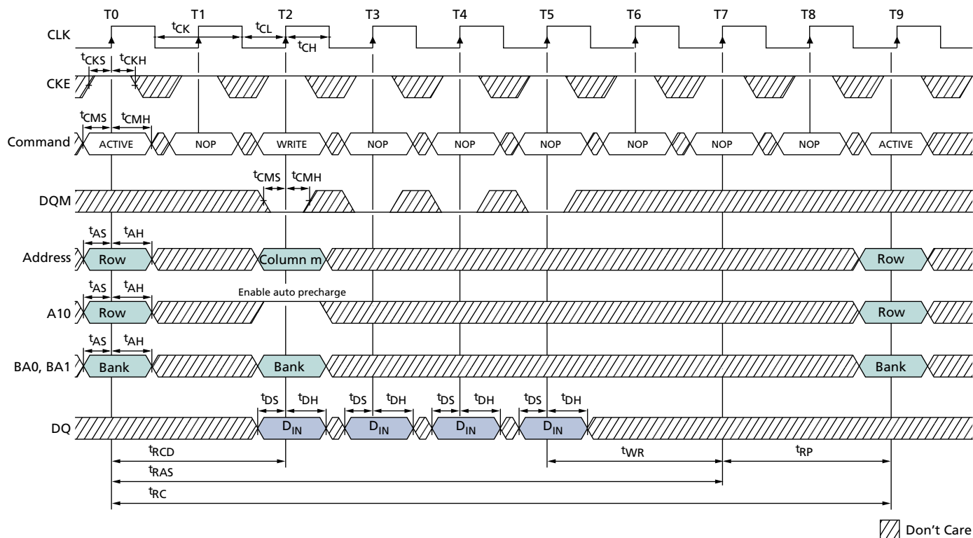
Figure 41: WRITE With Auto Precharge
