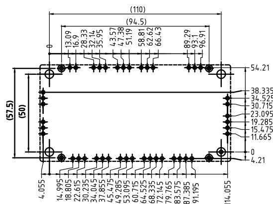
PCB hole pattern
