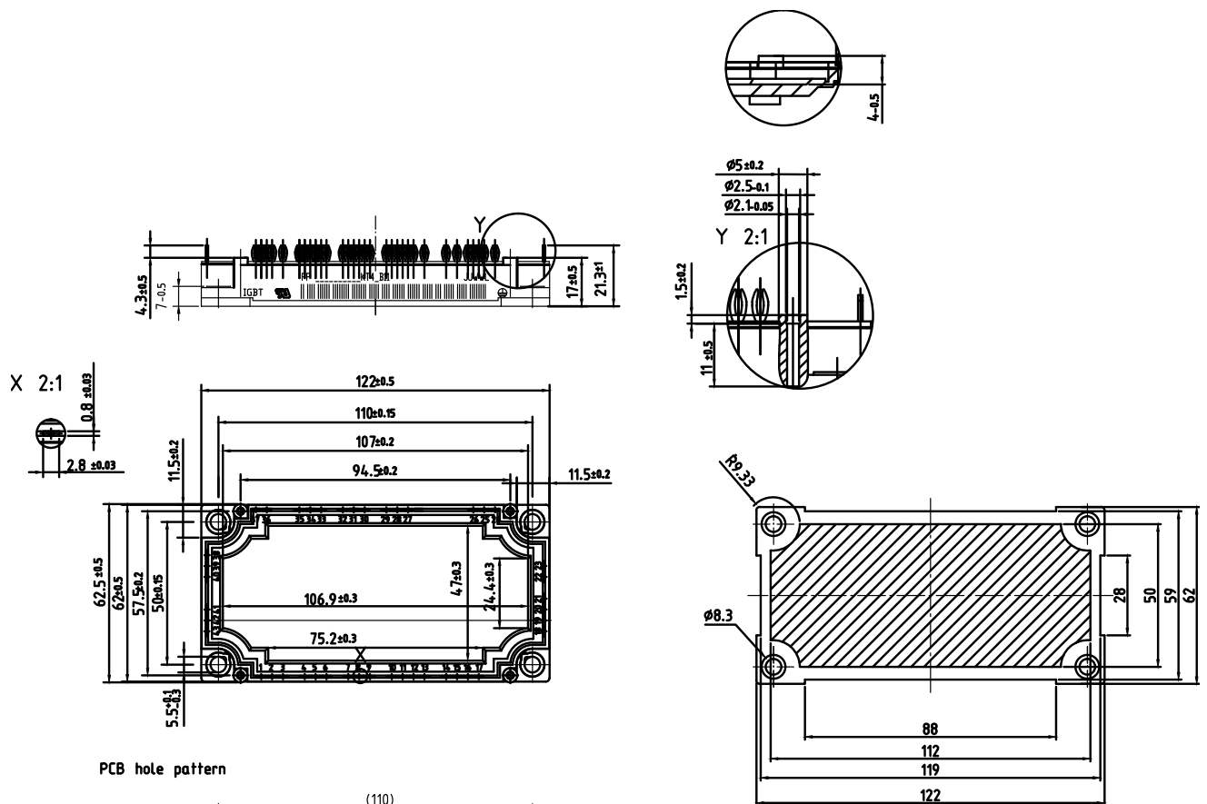
restricted area for Thermal Interface Material
