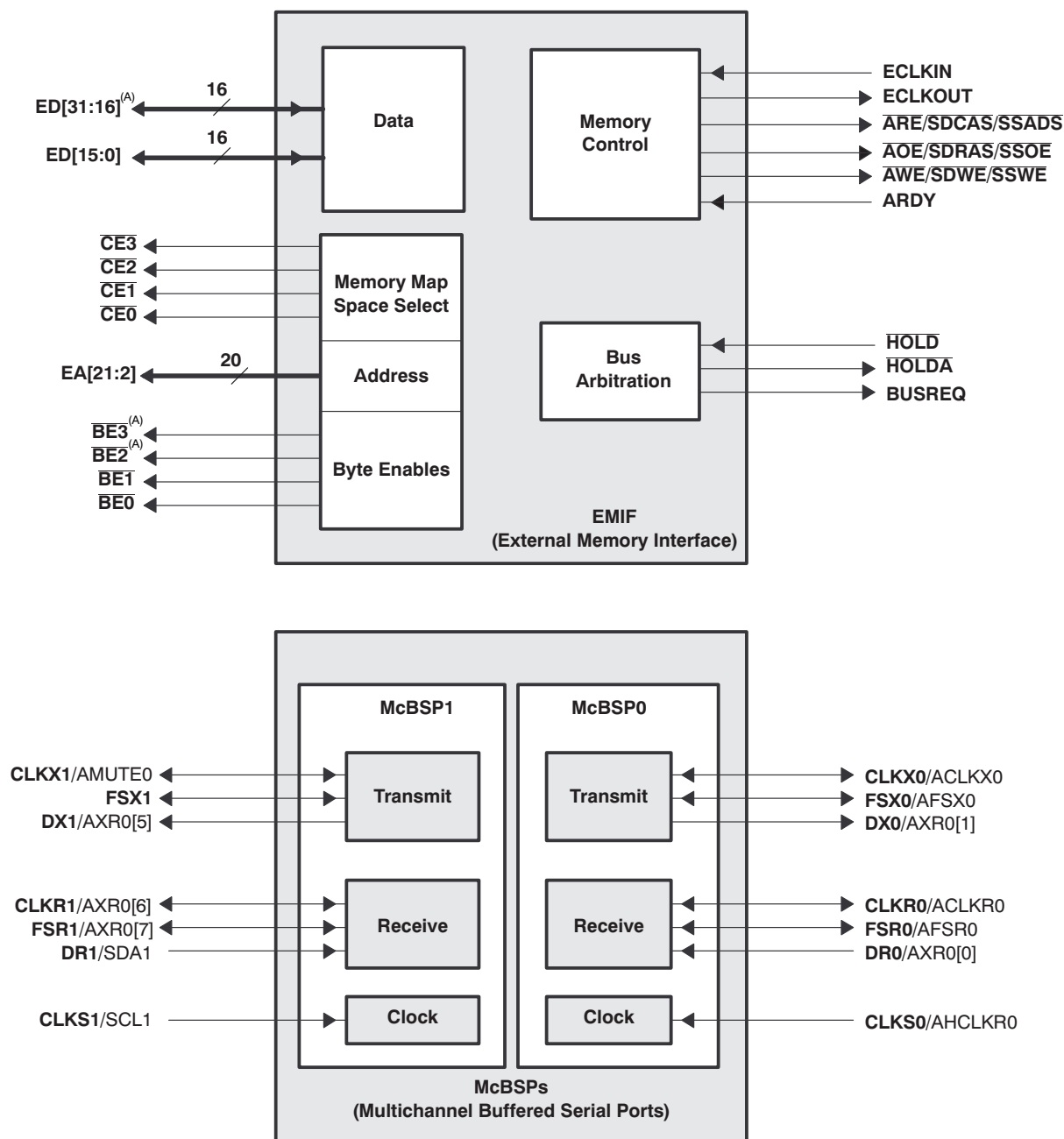
Figure 4-6. Peripheral Signals
