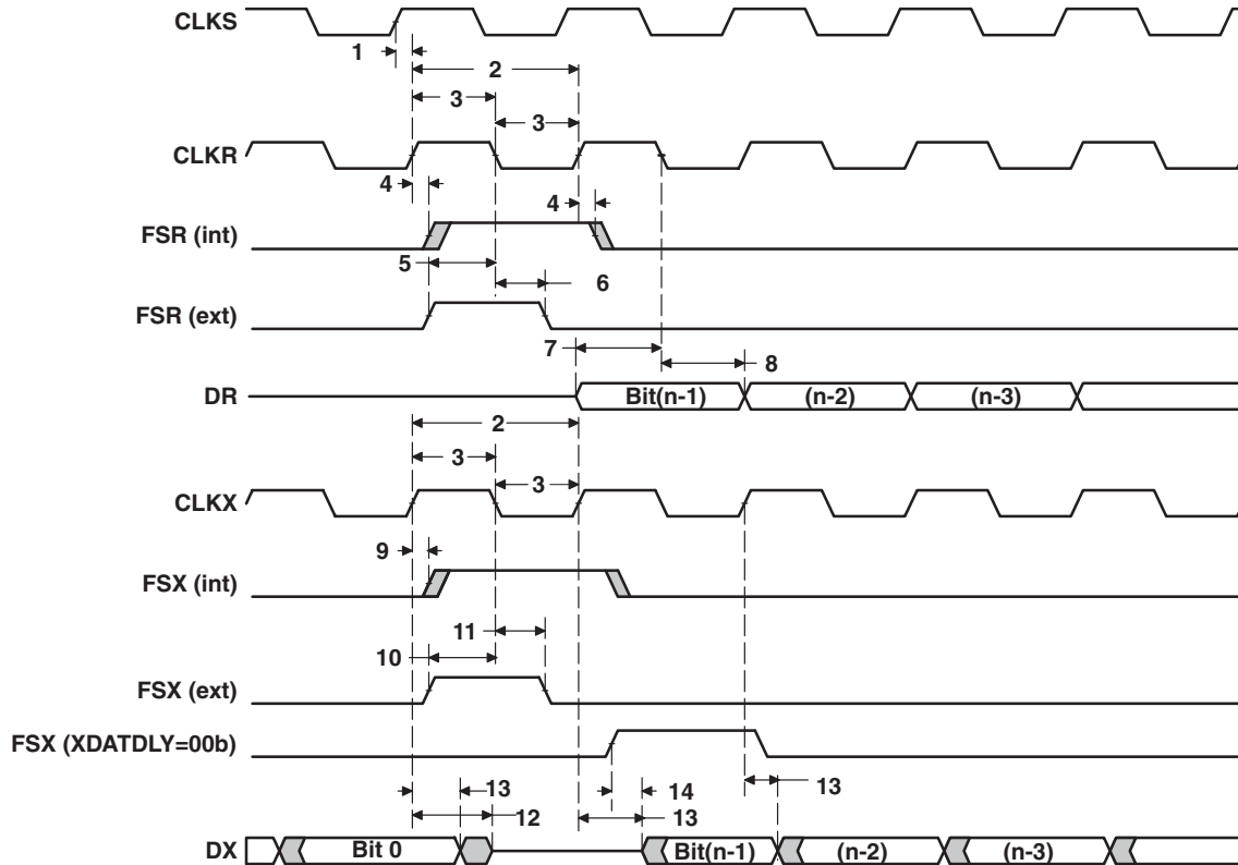
Figure 11-35. McBSP Timings
