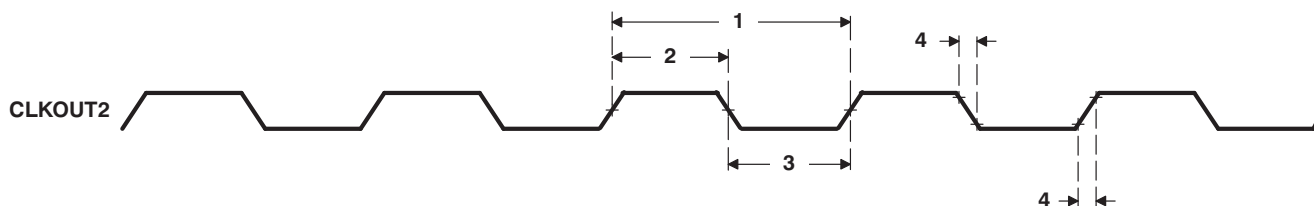
Figure 11-8. CLKOUT2
