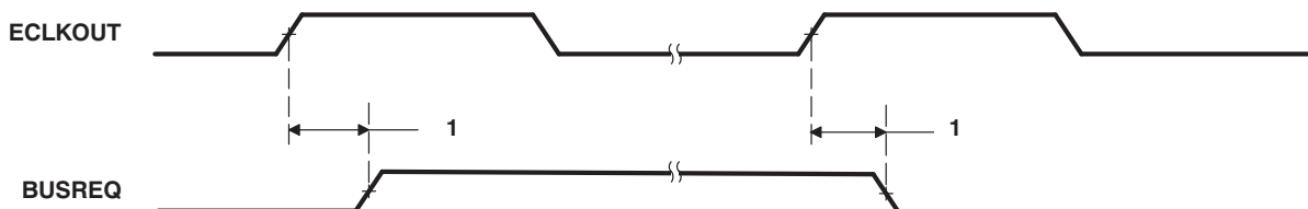
Figure 11-24. BUSREQ
