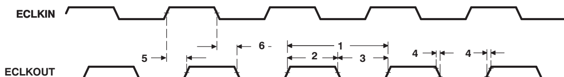
Figure 11-11. ECLKOUT
