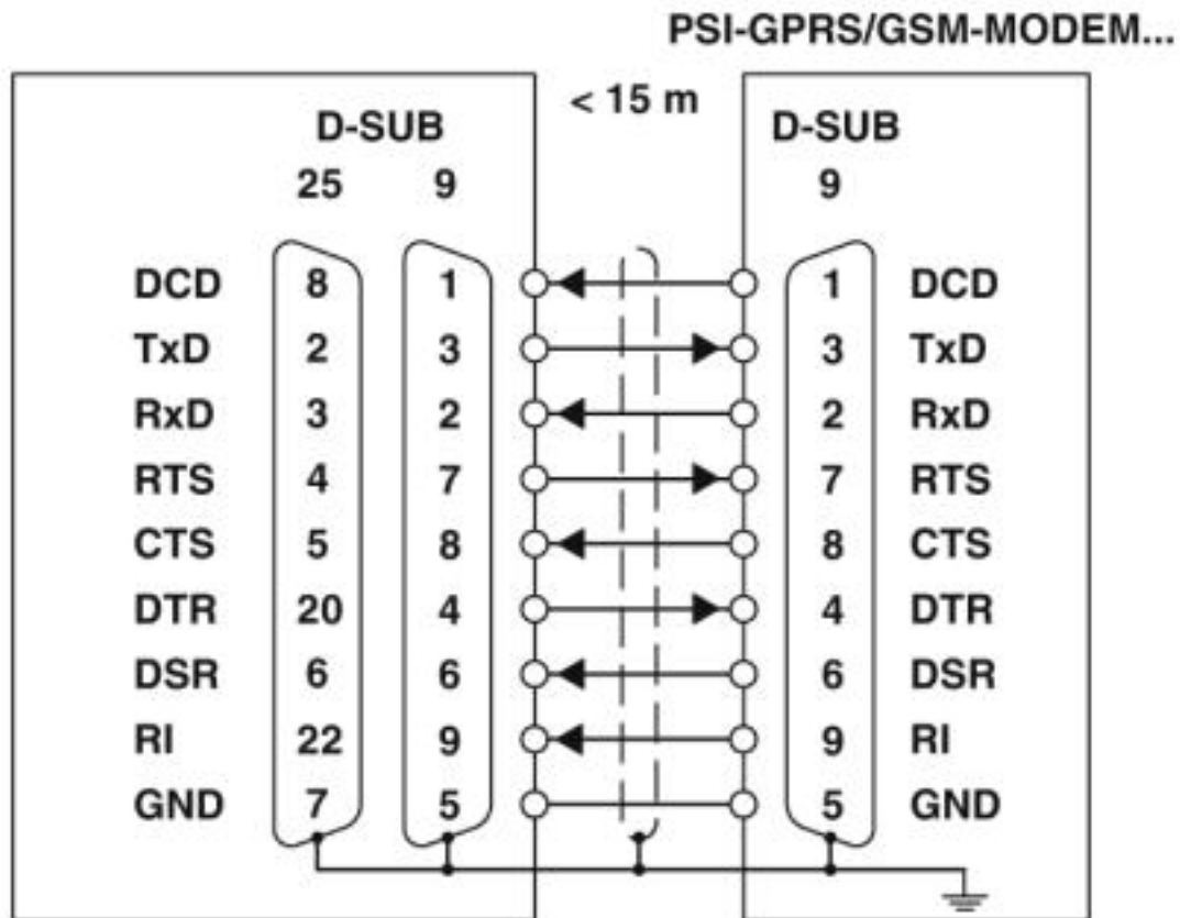
Connection diagram
