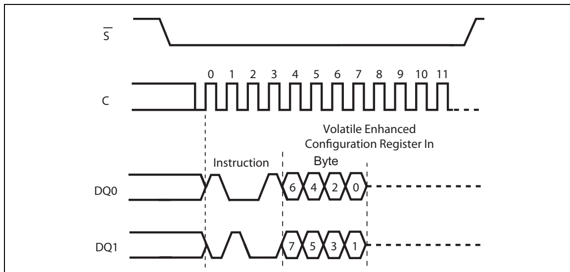
Figure 67. Write Volatile Enhanced Configuration Register instruction sequence PIQ-SPI
