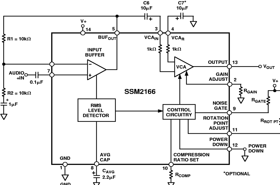
Figure 14. Functional Block Diagram and Typical Application
