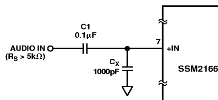
Figure 21. Circuit Configuration for Use with High Impedance Signal Sources
