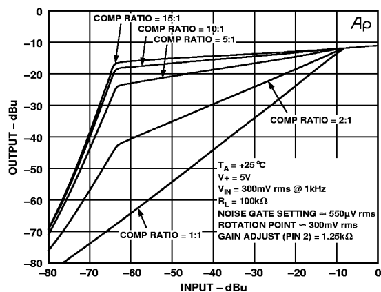
Figure 3. Output vs. Input Characteristics
