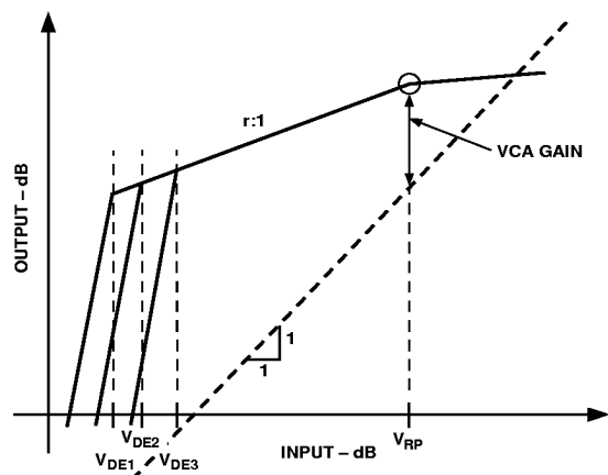
Figure 20. Effect of Varying the Downward Expansion (Noise Gate) Threshold
