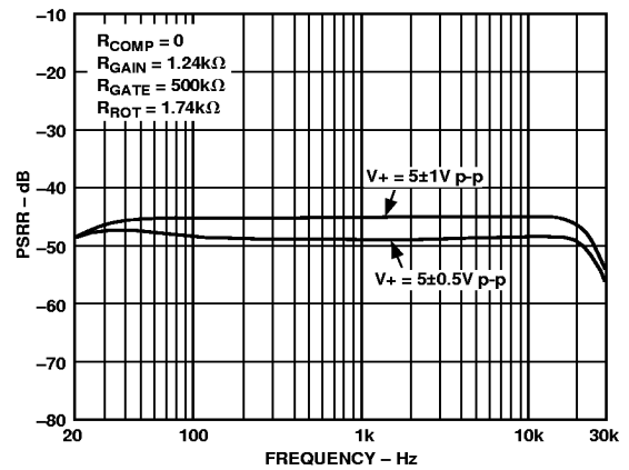
Figure 10c. PSRR vs. Frequency
