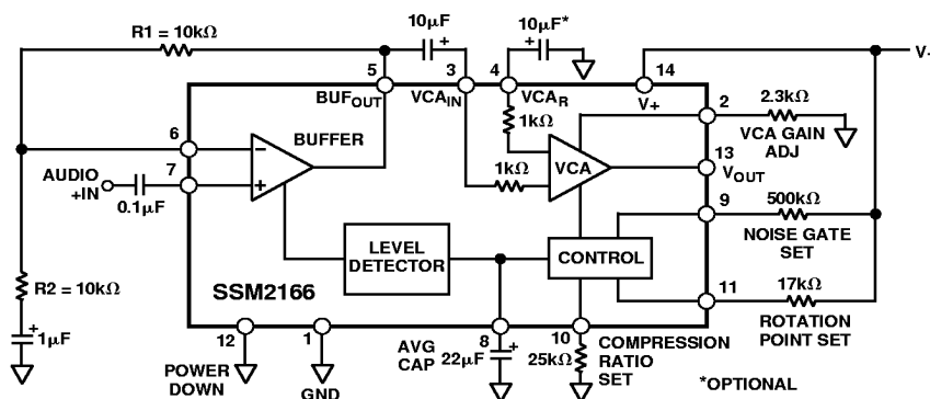
Figure 2. Functional Block Diagram and Typical Speech Application
