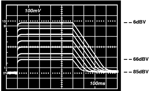
Figure 15a. RMS Level Detector Performance with C_{AVG} = 2.2 \mu F
