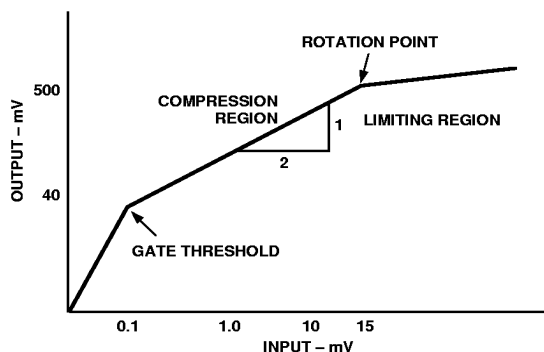
Figure 25. Transfer Characteristic
