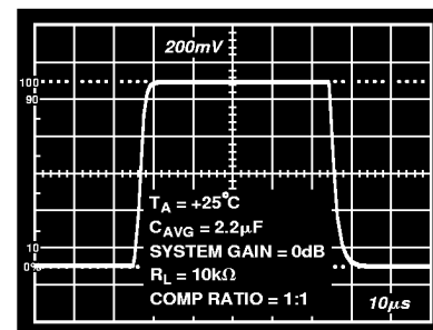
Figure 12. Large Signal Transient Response
