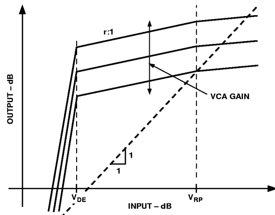
Figure 18. Effect of Varying the VCA Gain Setting
