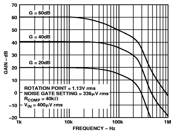
Figure 10b. GBW Curves vs. VCA Gain
