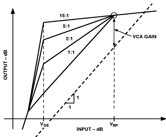
Figure 16. Effect of Varying the Compression Ratio
