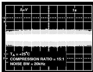
Figure 10a. Wideband Output Noise
