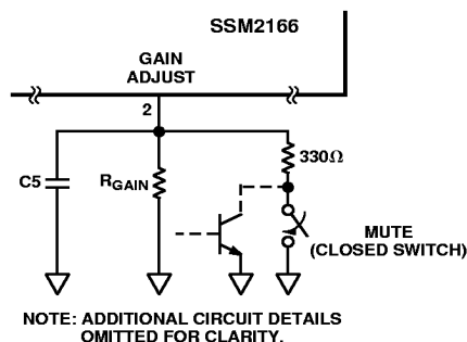
Figure 19. Details of SSM2166 Mute Option
