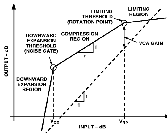
Figure 13. General Input/Output Characteristics of the SSM2166
