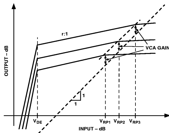
Figure 17. Effect of Varying the Rotation Point
