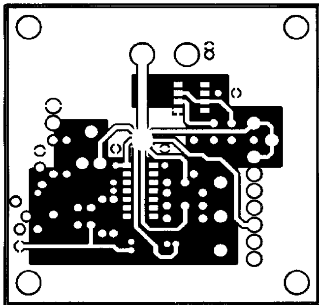
Figure 23b. Evaluation Board Topside Metallization (Not to Scale)
