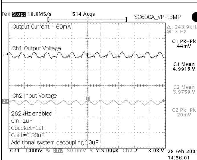
Ripple Voltage
