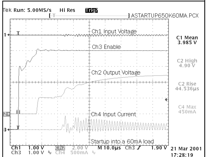
Startup Conditions for 5.0V Output
