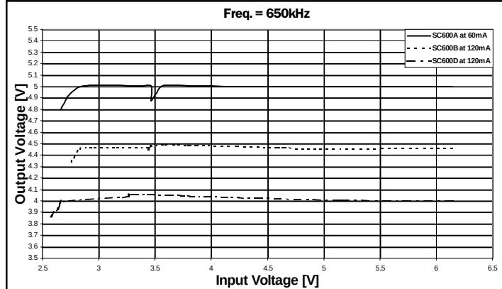
Line Regulation
