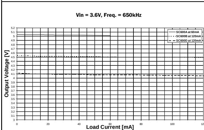
Load Regulation
