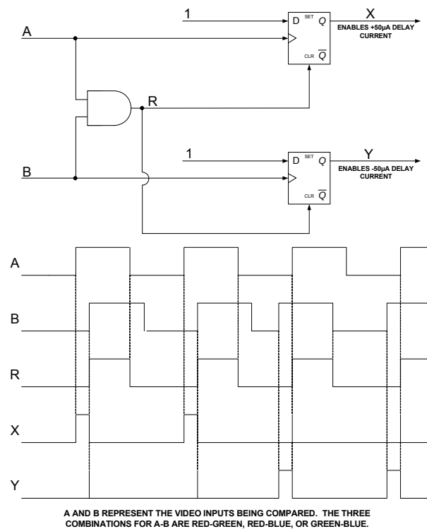
FIGURE 15. DELAY DETECTOR
