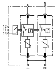
Basic circuit diagram DG M TN ... FM
