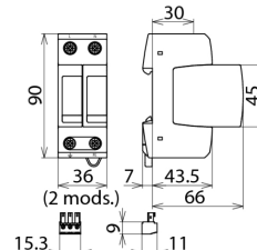
Dimension drawing DG M TN ... FM
