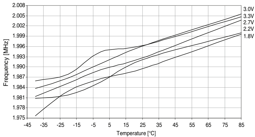
Figure 37-321. 2MHz internal oscillator frequency vs. temperature.
