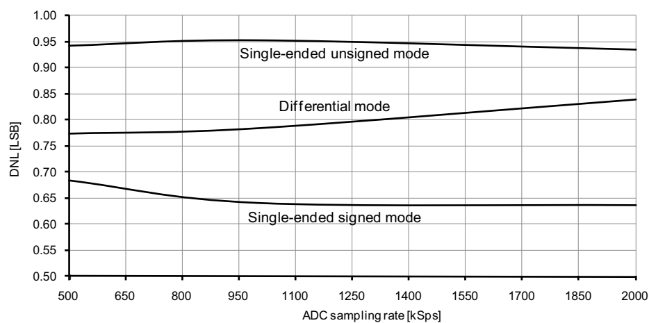
Figure 37-122. DNL error vs. sample rate.
