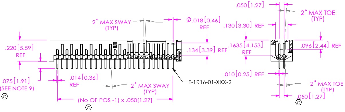
SECTION "B"-"B"
