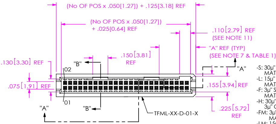
FIG 1 -01: THROUGH HOLE
