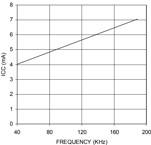
Graph 5: ICC vs Frequency
