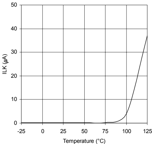
Graph 7: ILK vs TEMP
