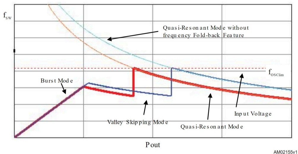
Figure 32. Switching frequency vs power
