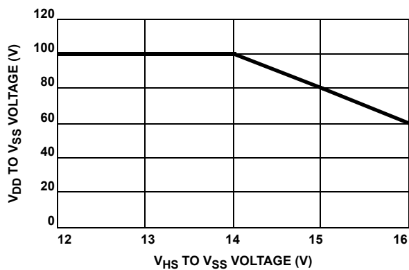
FIGURE 20. V_{HS} VOLTAGE vs V_{DD} VOLTAGE
