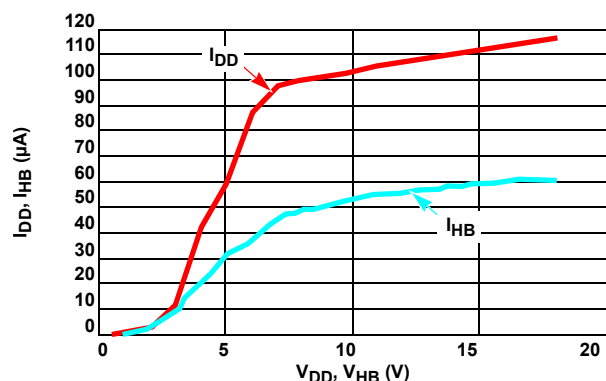
FIGURE 17. HIP2122 QUIESCENT CURRENT vs VOLTAGE
