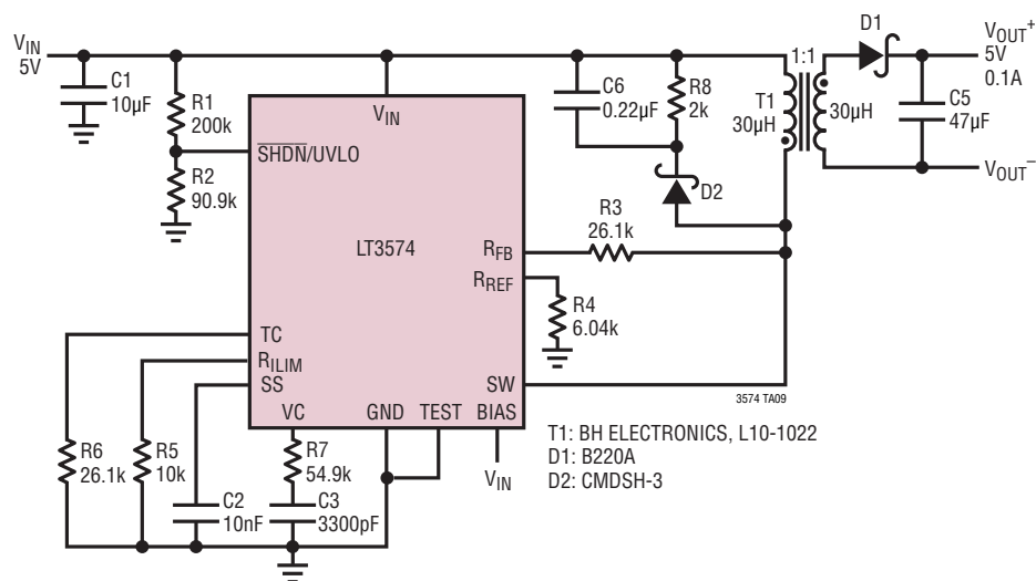
5V Isolated Flyback Converter Using Coupling Inductor
