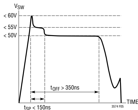
Figure 5. Maximum Voltages for SW Pin Flyback Waveform
