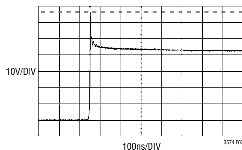
Figure 7. Bad Snubber Diode Does Not Limit SW Pin Voltage
