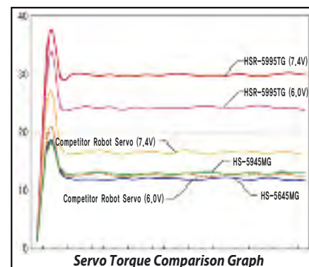
Servo Torque Comparison Graph
