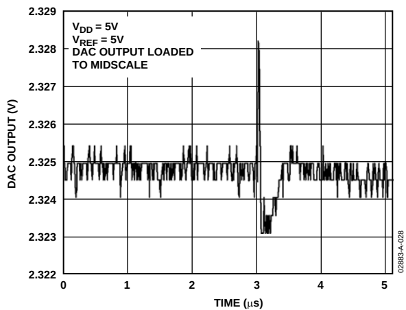
Figure 29. DAC-to-DAC Crosstalk
