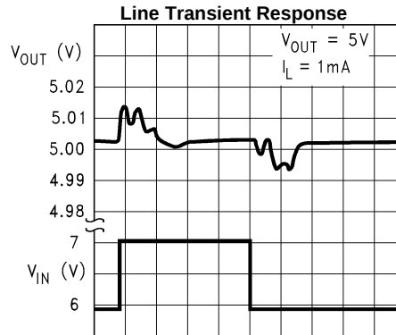
20 \mu\text{s}/\text{div} → Figure 17.
