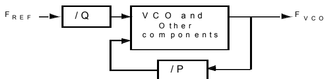
Figure 4. PLL system
