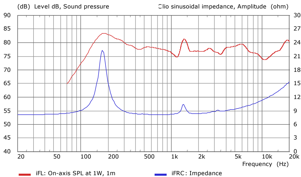
Figure 1. Impedance vs. frequency and SPL
