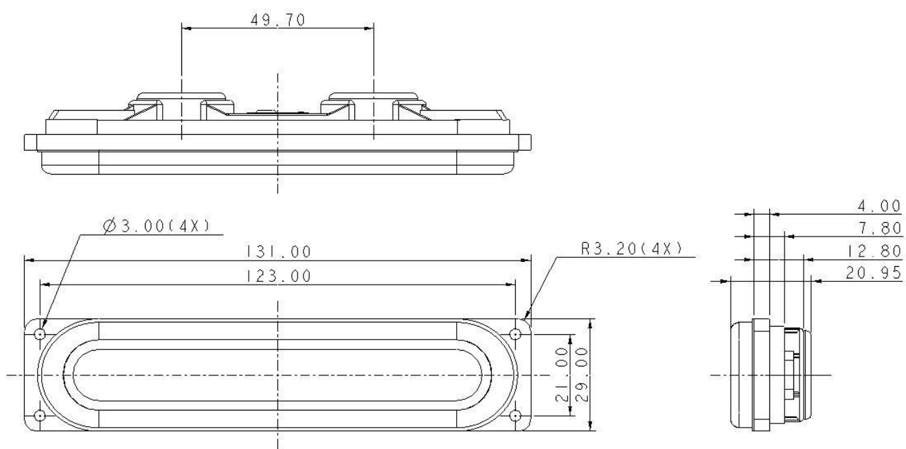
Figure 2. Nominal dimensions
