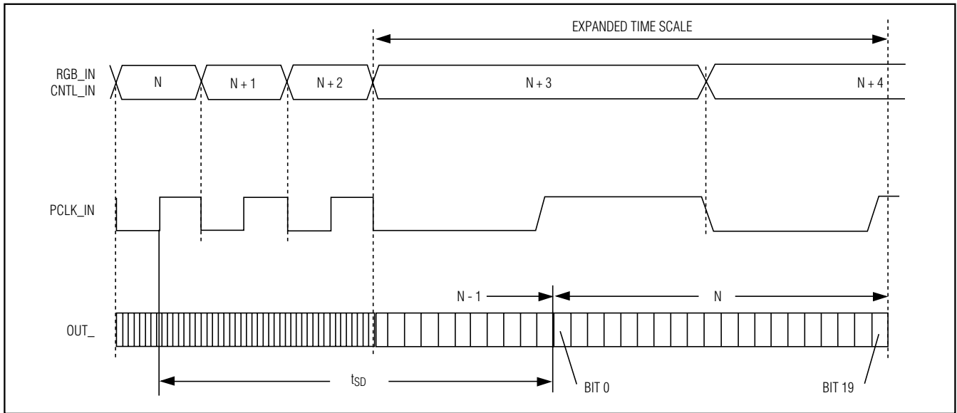
Figure 5. Serializer Delay
