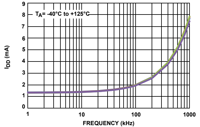
FIGURE 4. I_{DD} OPERATING CURRENT vs FREQUENCY, R_{DT} = 47\text{k}\Omega
