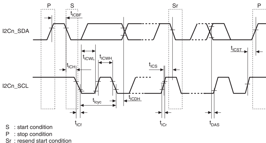
Figure 33.63 I 2 C Bus Interface Module Signal Timing
