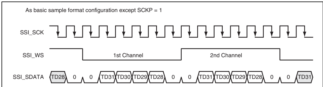
Figure 20.10 Inverted Clock
