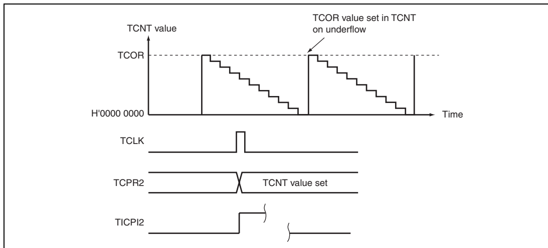
Figure 15.6 Operation Timing when Using Input Capture Function
