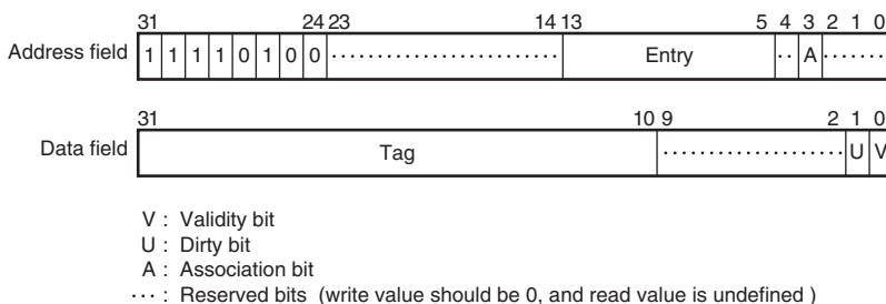
Figure 7.7 Memory-Mapped OC Address Array
