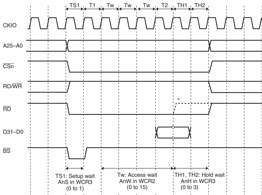
Figure 10.12 SRAM Interface Wait State Timing (Read Strobe Negate Timing Setting; AnS = 1, AnW = 011, AnH = 10)
