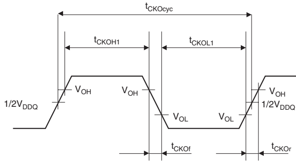
Figure 33.2 CKIO Clock Output Timing (1)
