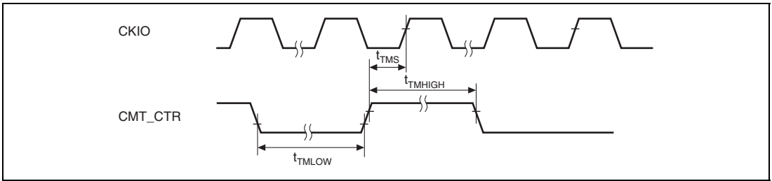
Figure 33.59 CMT Timing (2)
