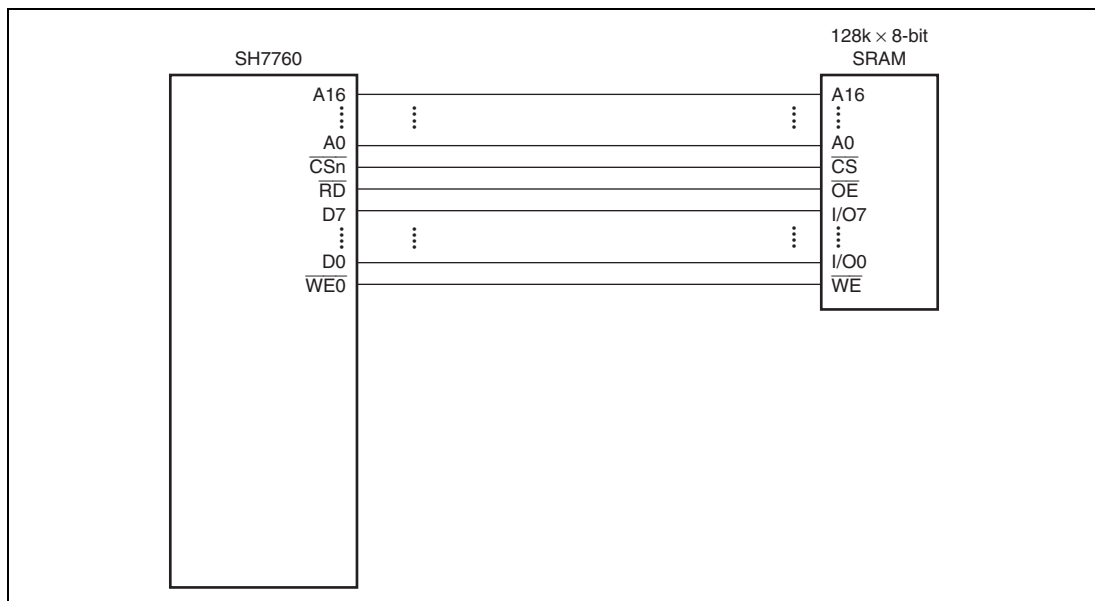
Figure 10.9 Example of 8-Bit Data Width SRAM Connection
