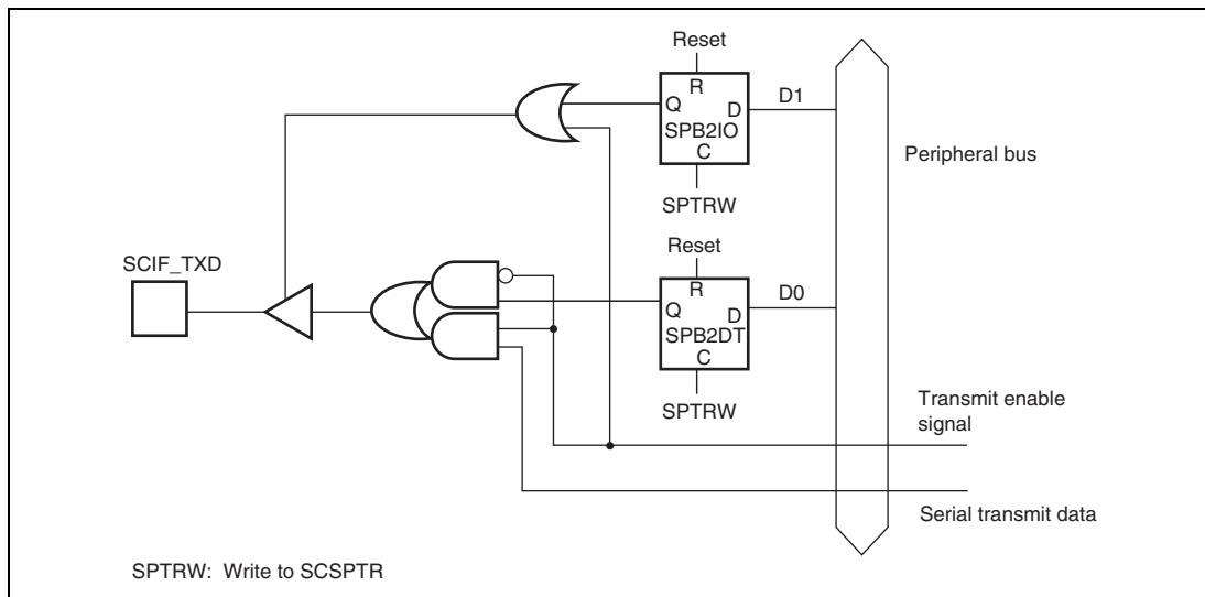
Figure 17.5 SCIF_TXD Pin
