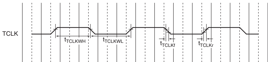
Figure 33.51 TCLK Input Timing
