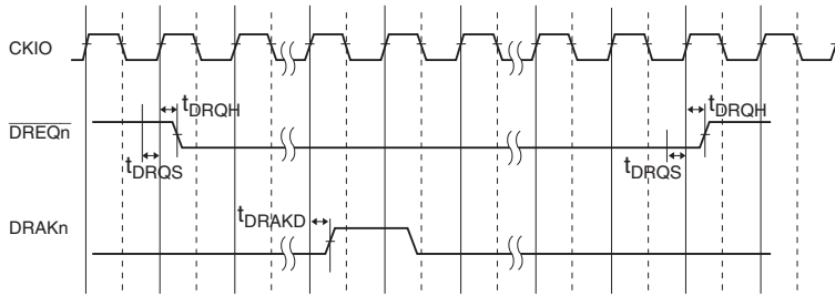
Figure 33.50 \overline{\text{DREQ}}/\text{DRAK} Timing
