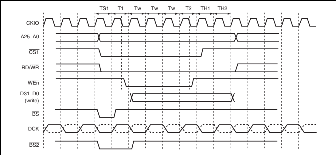
Figure 10.14 DCK, BS2, and CS1 Timing when Writing to SRAM Interface (DCKDR = H'0002, A1RDH = 1 and A1H[1:0] = 10 in WCR3, CSH[1:0] in WCR4 = 10, Three Wait Cycles)
