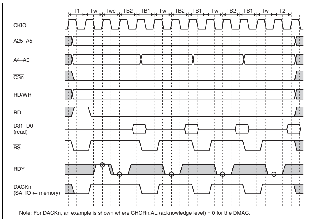
Figure 10.34 Burst ROM Wait Access Timing
