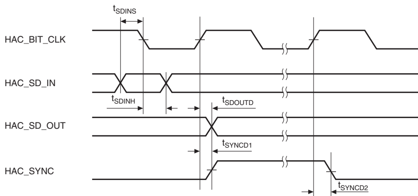
Figure 33.82 HAC Interface Module Signal Timing
