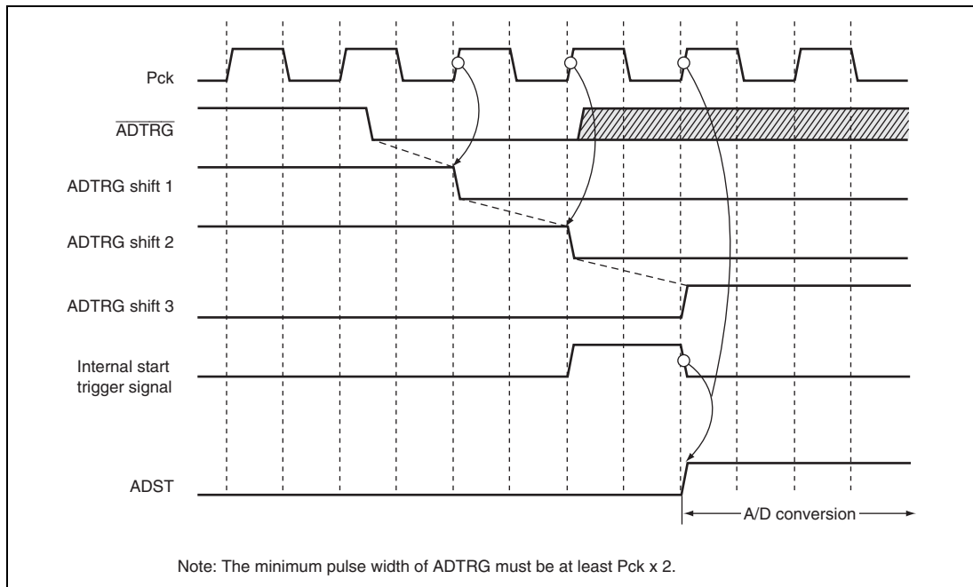
Figure 29.6 External Trigger Input Timing
