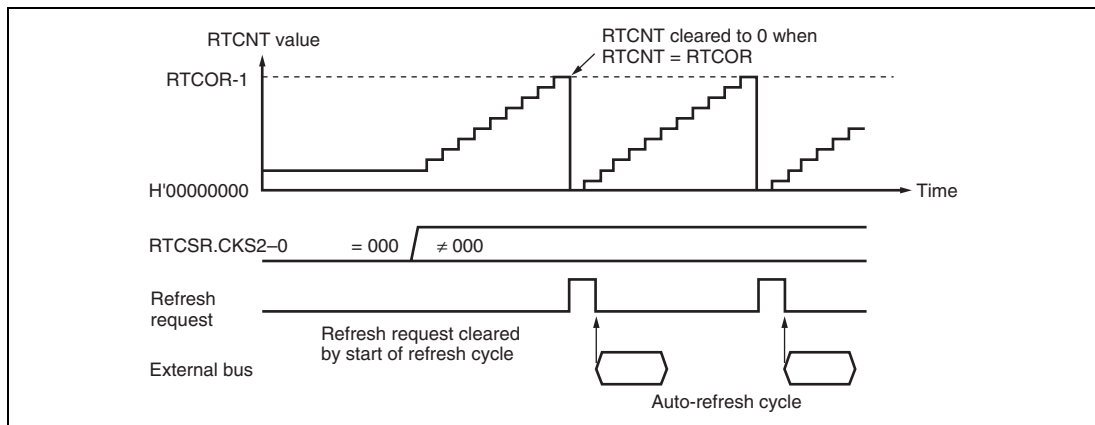
Figure 10.27 Auto-Refresh Operation
