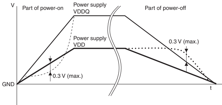
Figure F.1 Power-on and Power-off Procedure (1)
