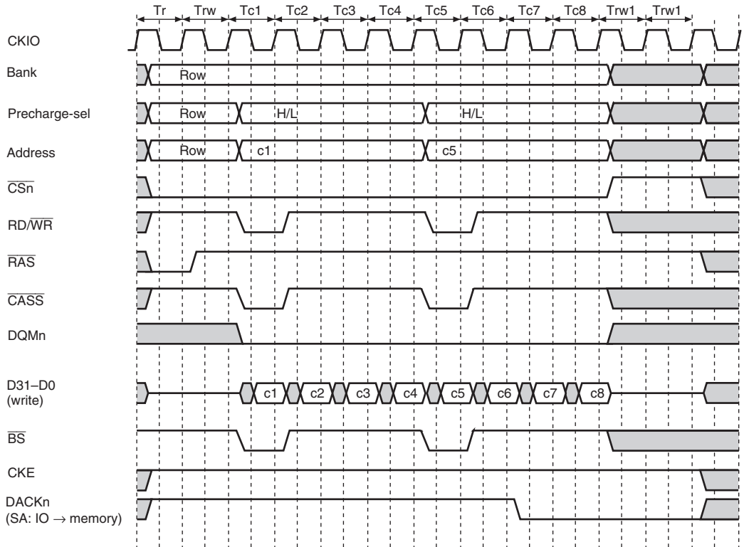
Figure 10.23 Burst Write Timing
