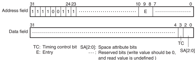
Figure 6.14 Memory-Mapped ITLB Data Array 2
