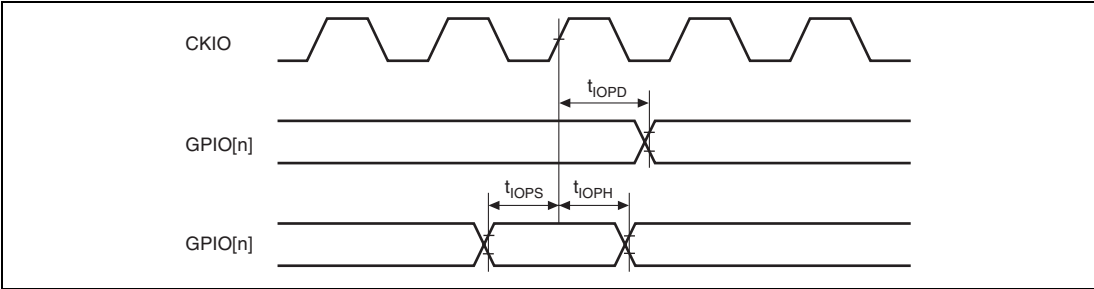
Figure 33.61 GPIO Timing
