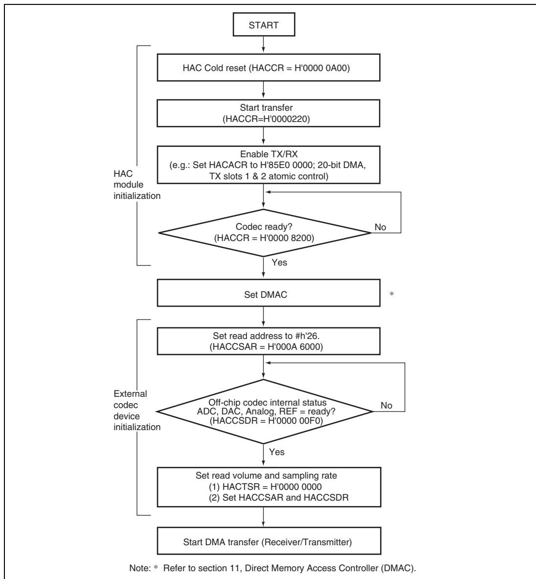
Figure 25.3 Initialization Sequence
