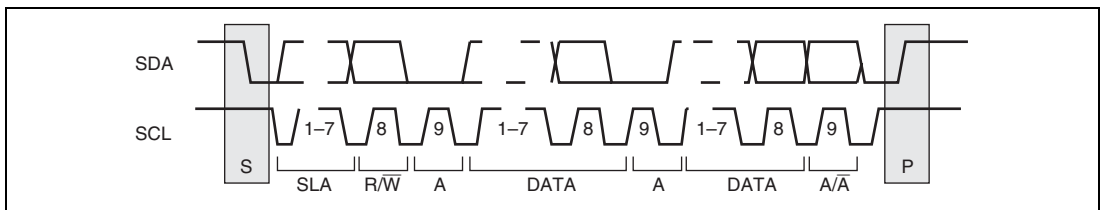
Figure 19.2 I 2 C Bus Timing
