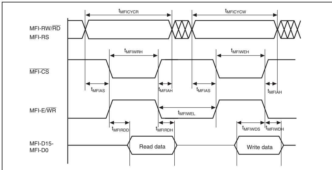
Figure 33.72 AC Characteristics of 68 Series Bus
