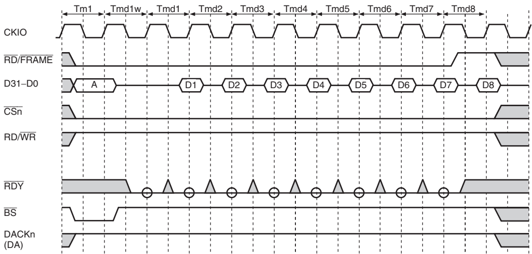
Figure 10.48 MPX Interface Timing 5 (Burst Read Cycle, AnW = 0, No External Wait, 32-Bit Bus Width, 32-Byte Data Transfer)
