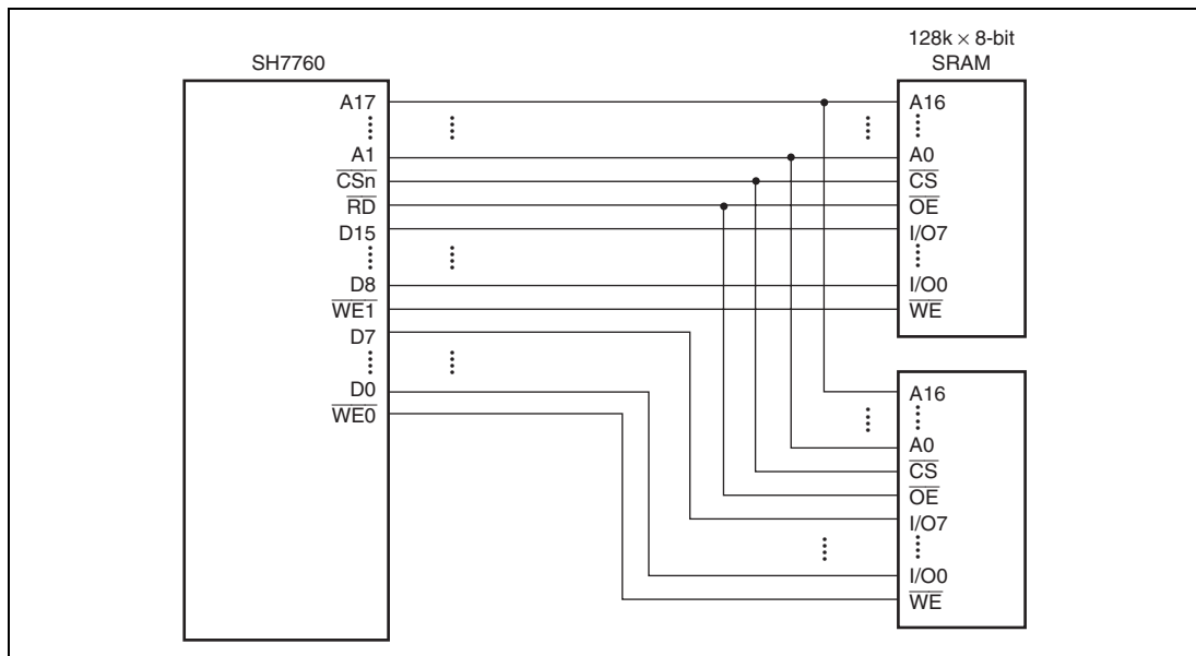
Figure 10.8 Example of 16-Bit Data Width SRAM Connection
