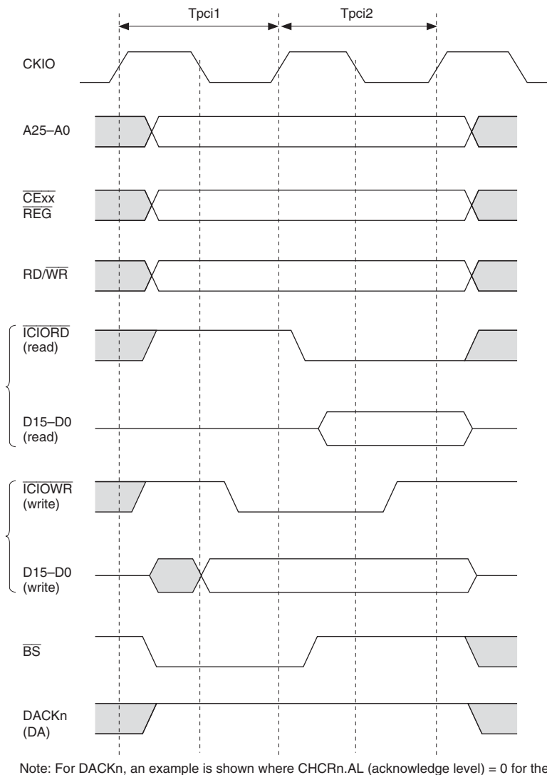
Figure 10.40 Basic Timing for PCMCIA I/O Card Interface
