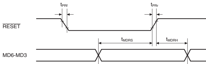
Figure 33.14 MD pins Setup/Hold Timing
