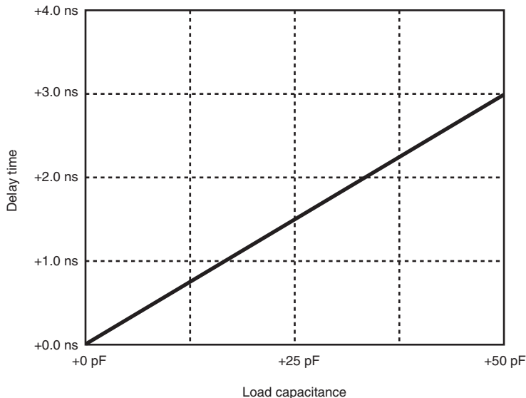
Figure 33.89 Load Capacitance-Delay Time
