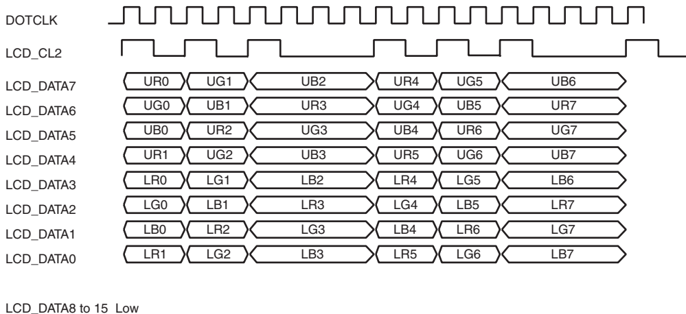
Figure 30.16 Clock and LCD Data Signal Example
