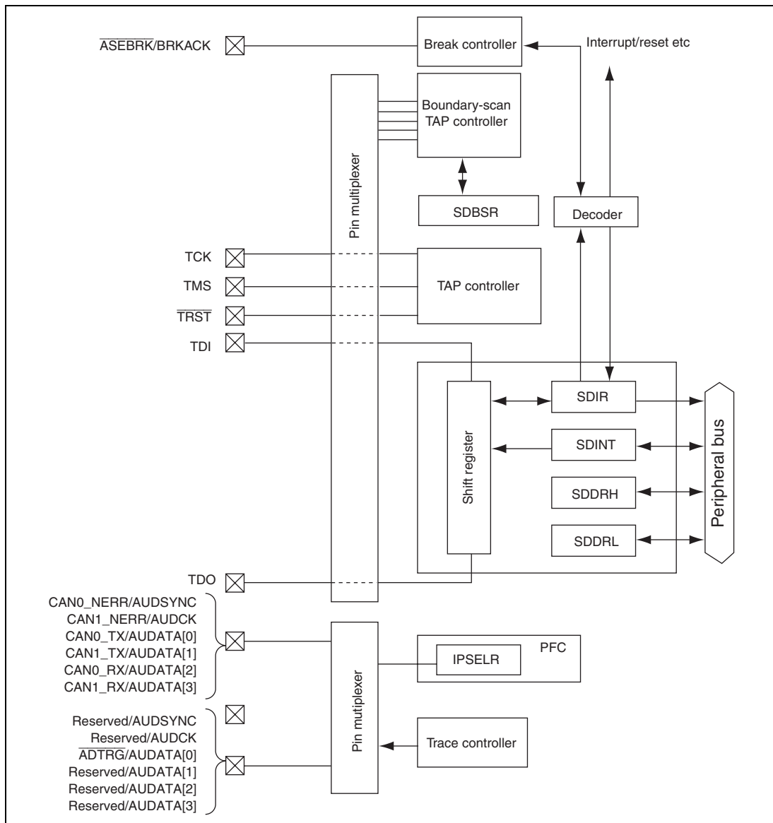
Figure 28.1 H-UDI Block Diagram
