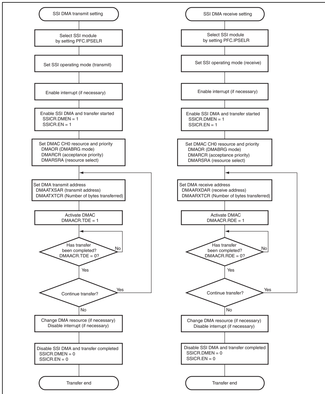
Figure 11.33 Example of SSI DMA Transfer Operation Flow
