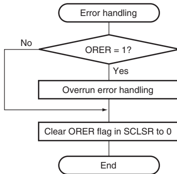
Figure 17.19 Sample Serial Reception Flowchart (2)
