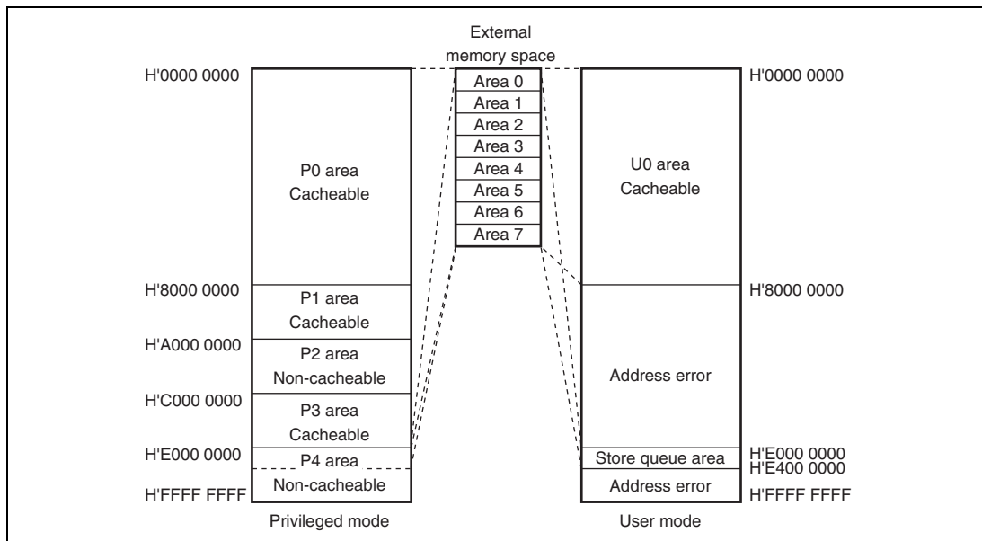
Figure 6.2 Physical Address Space (AT = 0 in MMUCR)
