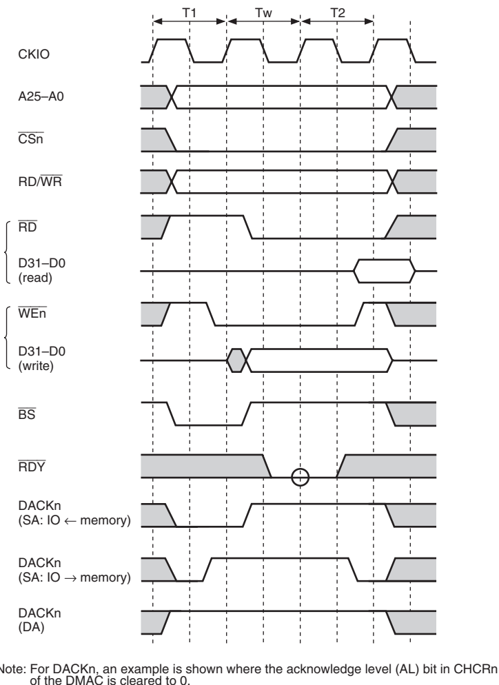
Figure 10.10 SRAM Interface Wait Timing (Software Wait Only)
