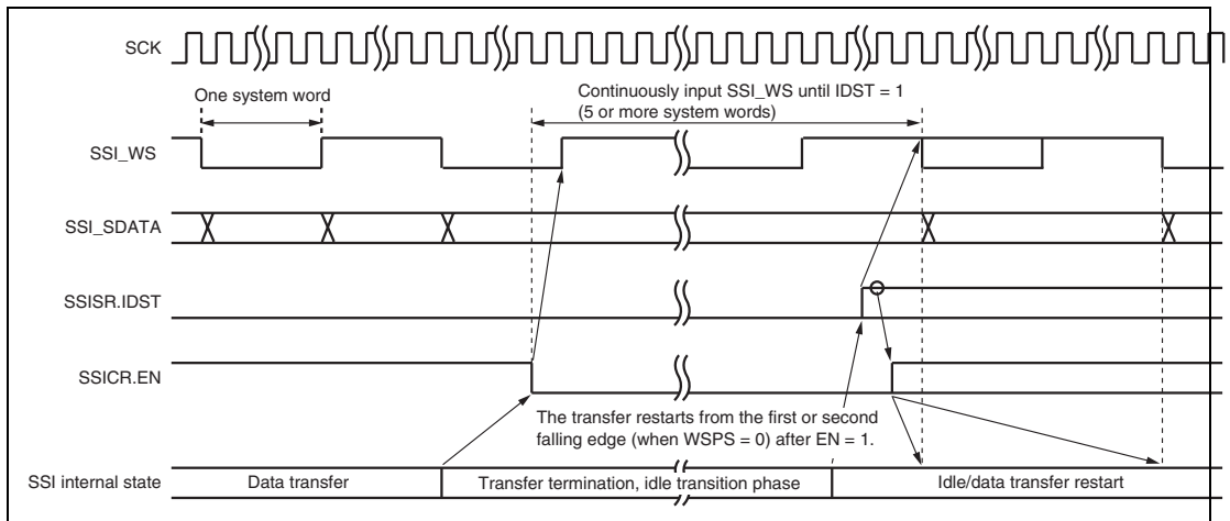
Figure 20.25 Slave Mode SSI Transfer Termination/Restart Timing
