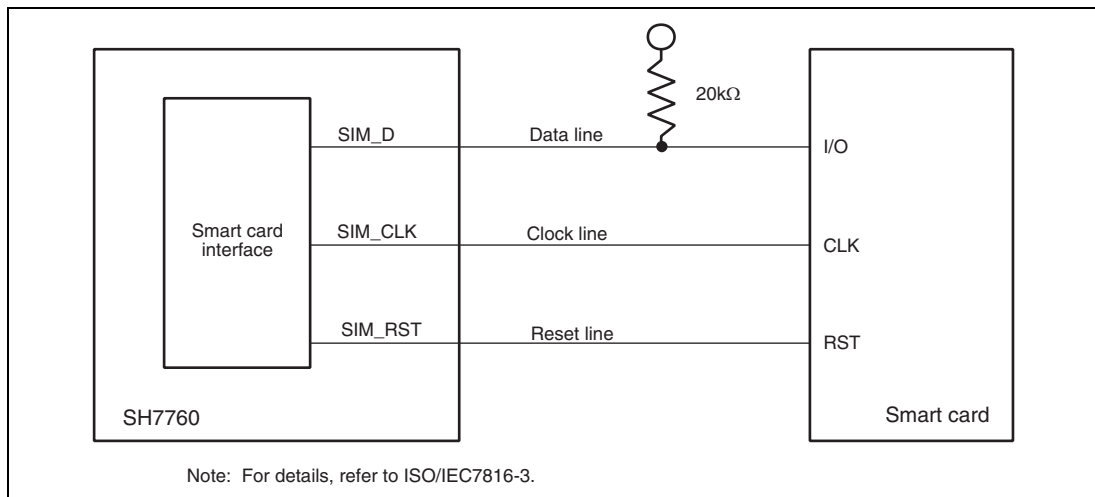
Figure 18.12 Example of Smart Card Interface Pin Connections
