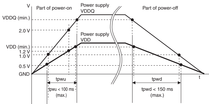
Figure F.2 Power-on and Power-off Procedure (2)
