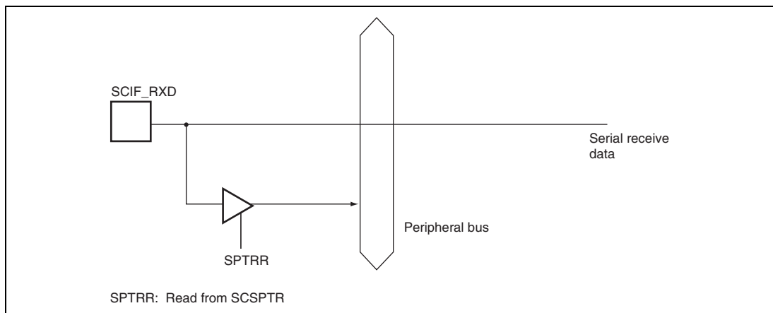
Figure 17.6 SCIF_RXD Pin
