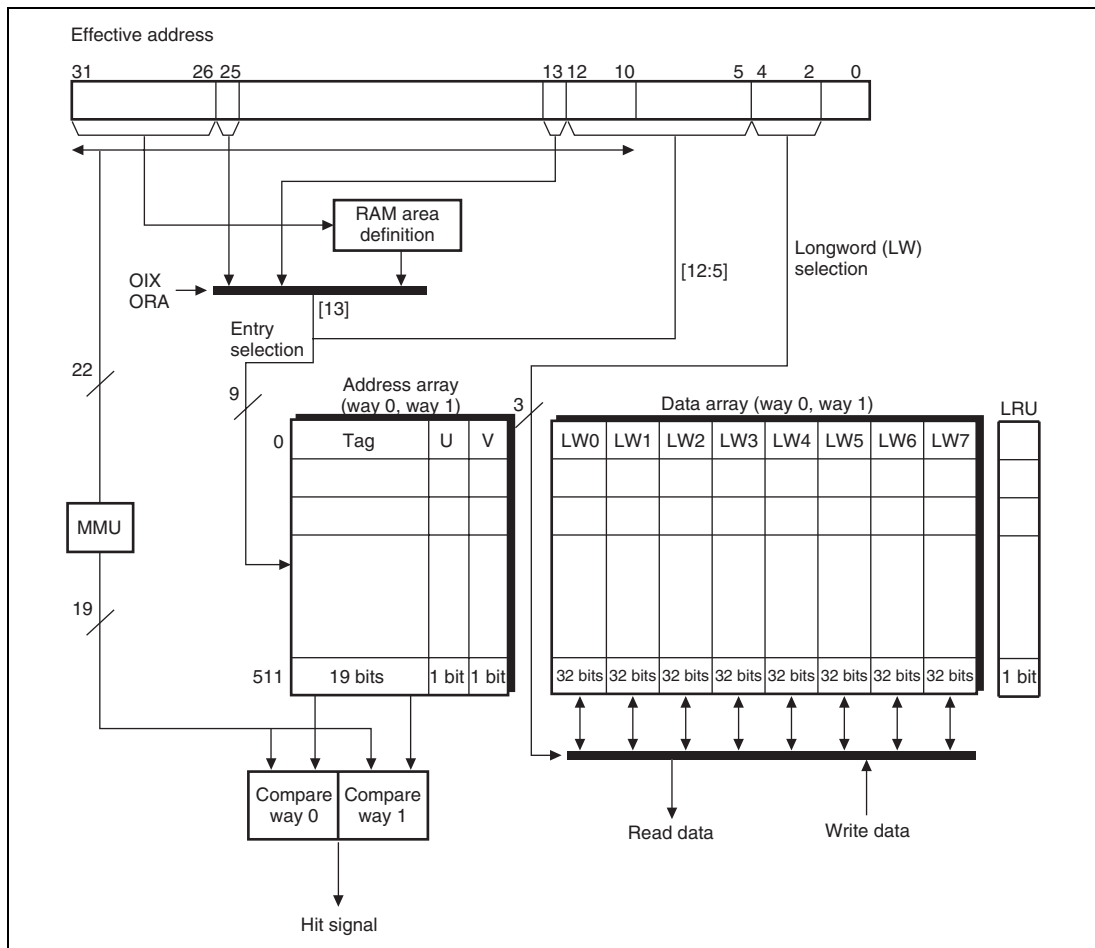
Figure 7.1 Configuration of Operand Cache
