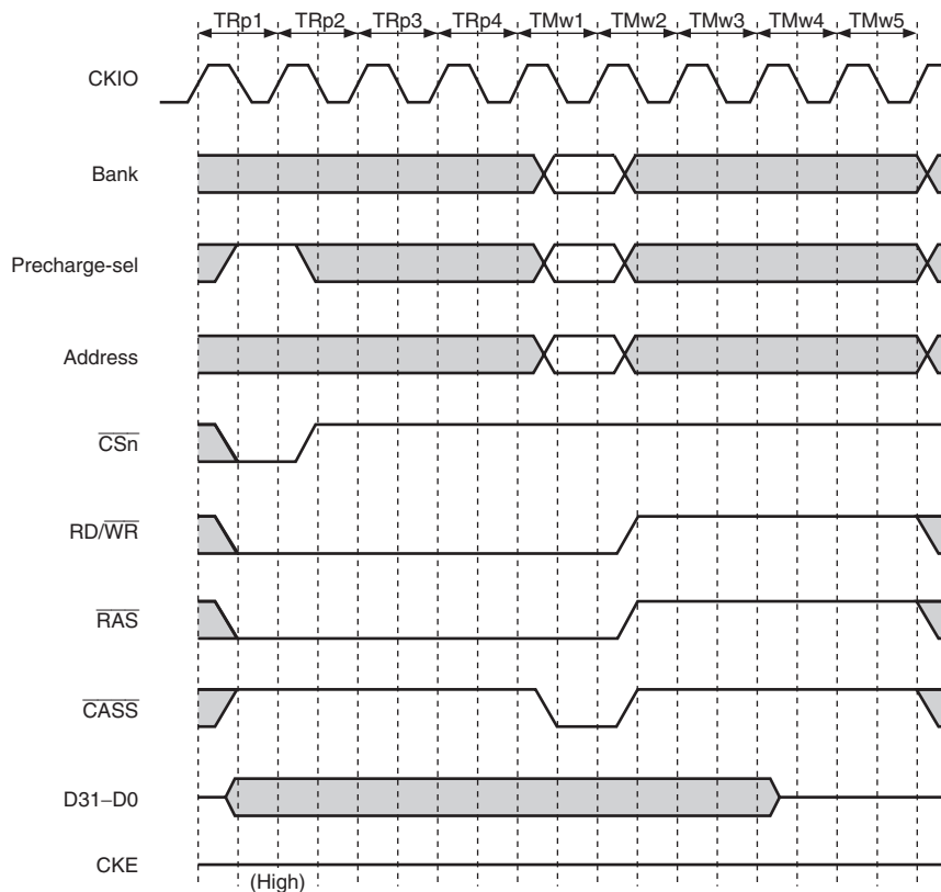
Figure 10.30 (1) Synchronous DRAM Mode Write Timing (PALL)
