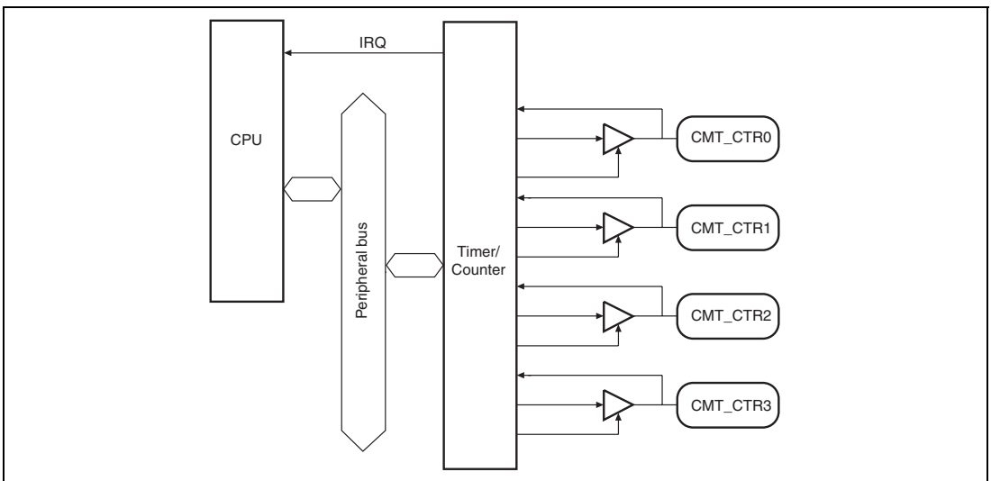
Figure 16.1 Block Diagram of CMT
