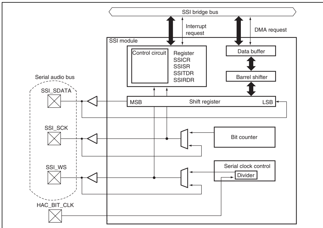
Figure 20.1 Block Diagram of SSI Module
