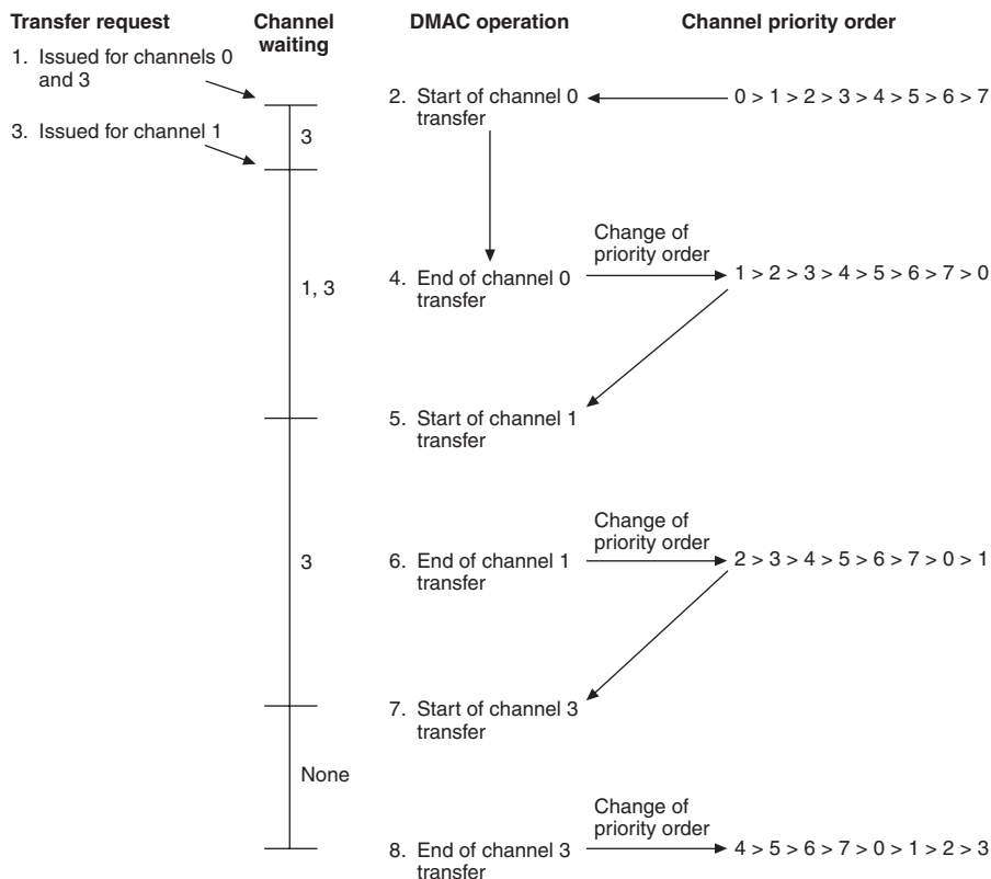
Figure 11.5 Example of Changes in Priority Order in Round Robin Mode
