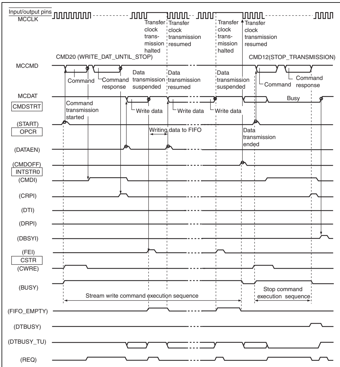
Figure 26.18 Example of Command Sequence for Commands with Write Data (Stream Transfer)
