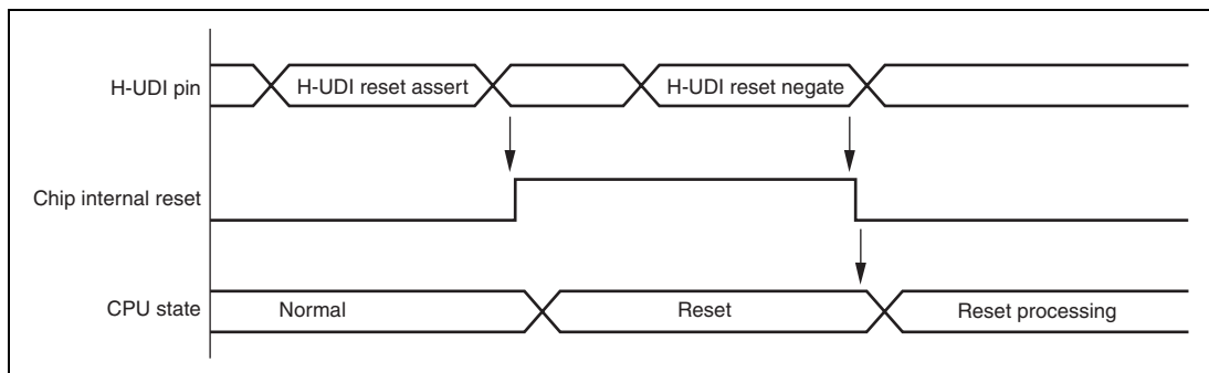
Figure 28.3 H-UDI Reset
