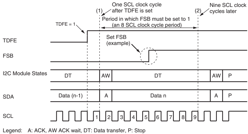
Figure 19.11 Period for Setting FSB = 1 for which a Stop Condition (P) will be Correctly Issued
