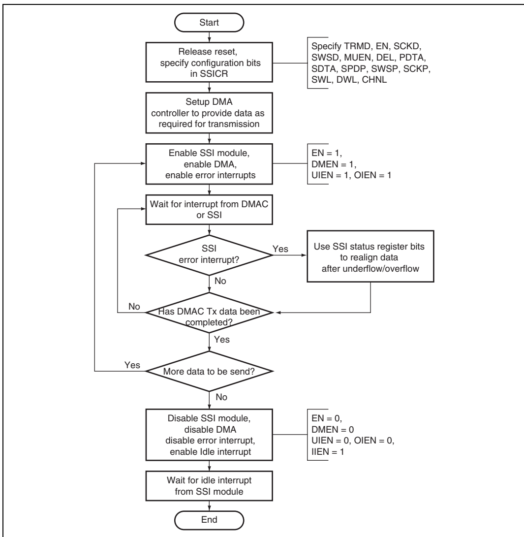
Figure 20.21 Transmission Using DMA Controller
