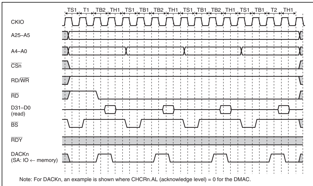
Figure 10.35 Burst ROM Wait Access Timing
