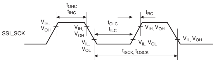
Figure 33.83 SSI Clock Input/Output Timing
