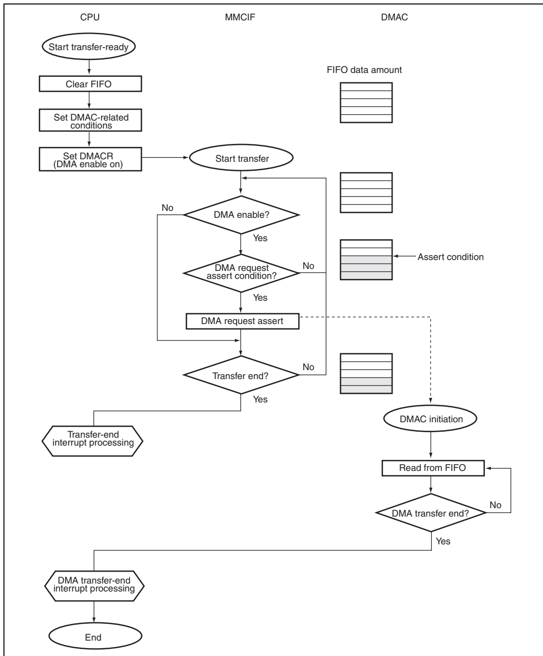
Figure 26.22 Example of Read Sequence Flow
