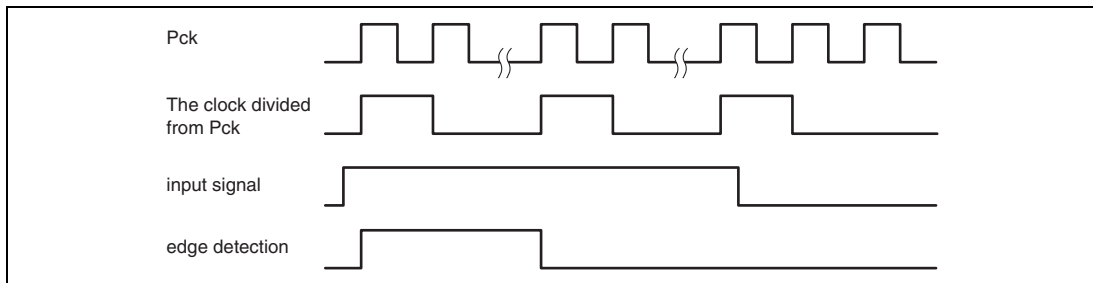
Figure 16.2 Edge Detection
