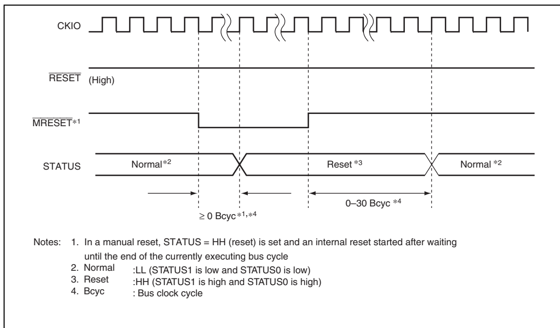
Figure 14.2 STATUS Output in Manual Reset
