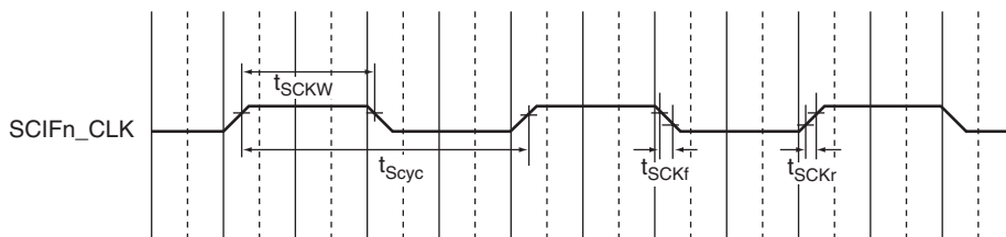
Figure 33.52 SCIFn_CLK Input Clock Timing
