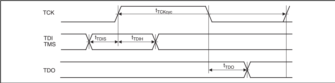
Figure 33.56 H-UDI Data Transfer Timing
