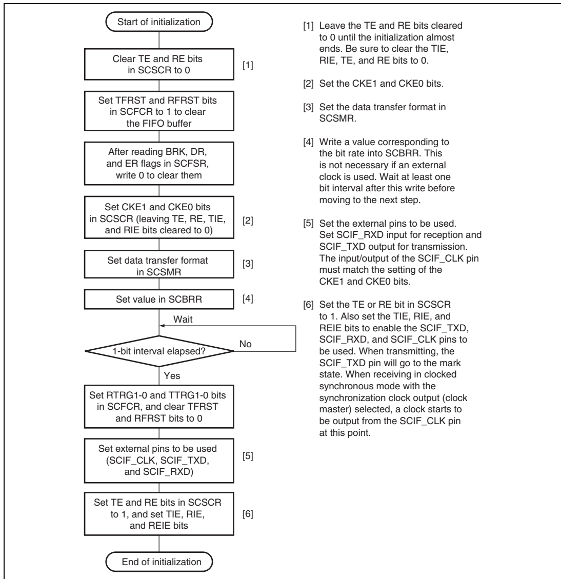
Figure 17.16 Sample SCIF Initialization Flowchart
