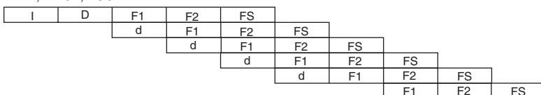
Figure 5.2 Instruction Execution Patterns (cont)
