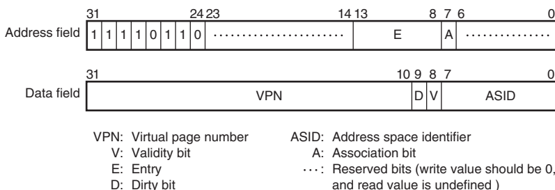
Figure 6.15 Memory-Mapped UTLB Address Array
