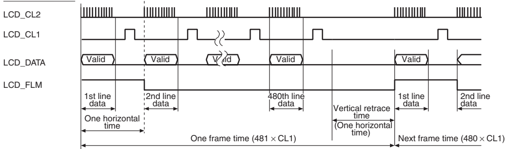
Figure 30.21 Clock and LCD Data Signal Example
