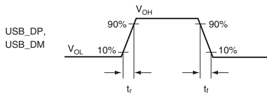
Figure 33.70 t_r , t_f
