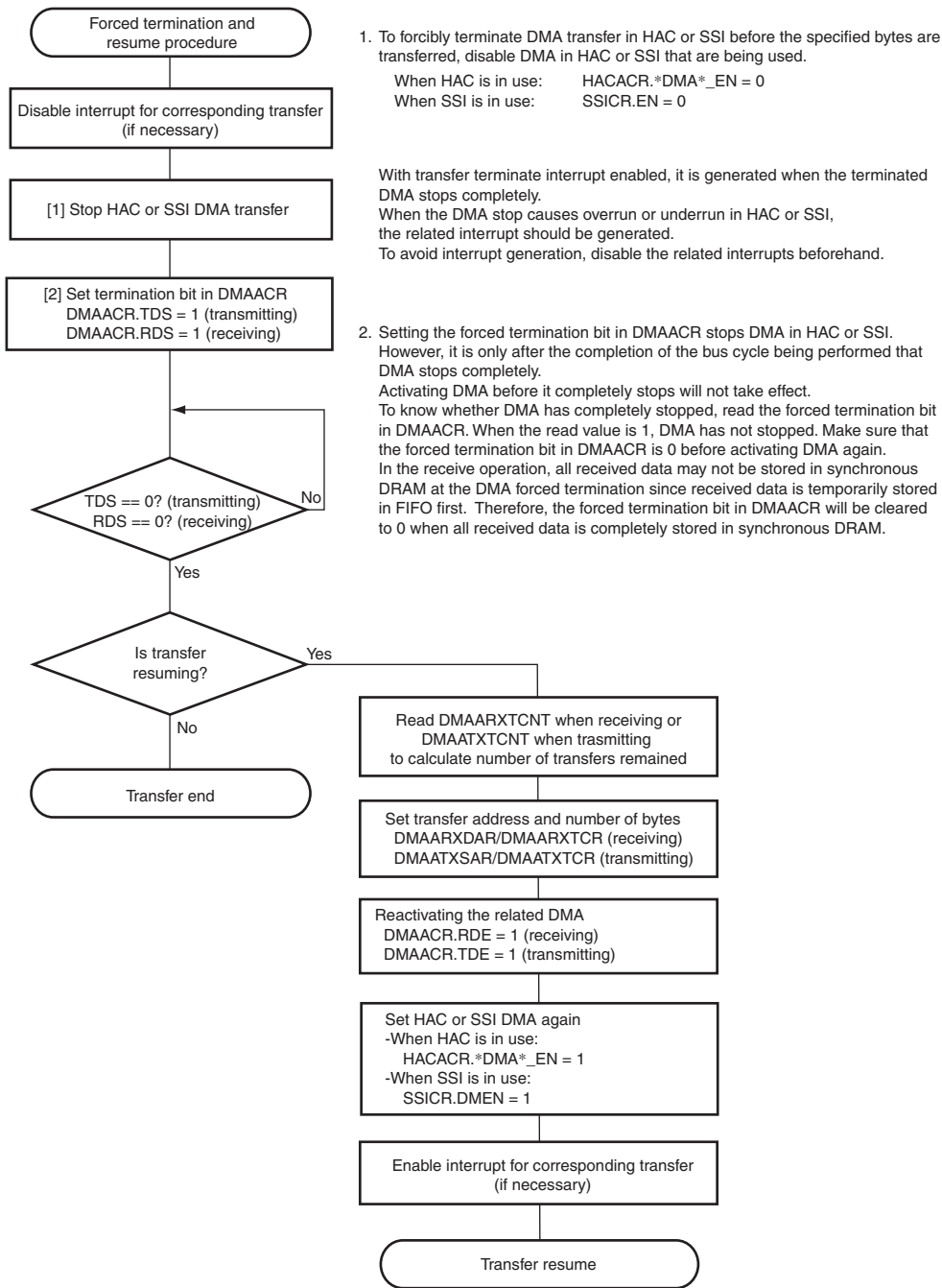
Figure 11.34 Forced Termination and Resume Procedures for DMA Audio Transfer
