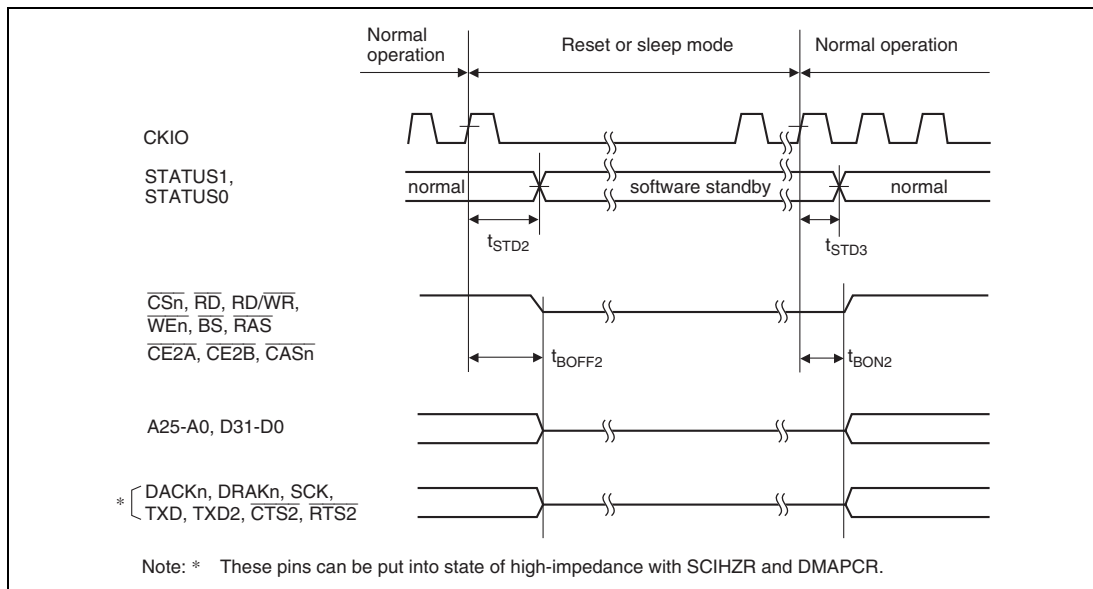
Figure 33.16 (2) Pin Drive Timing for Software Standby Mode
