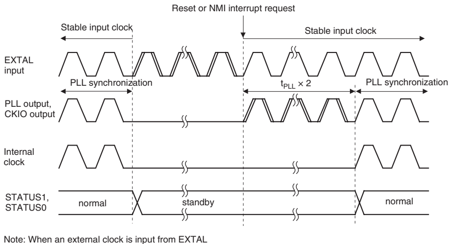
Figure 33.12 PLL Synchronization Settling Time in Case of RESET , MRESET or NMI Interrupt
