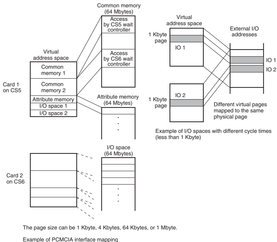
Figure 10.39 PCMCIA Space Allocation
