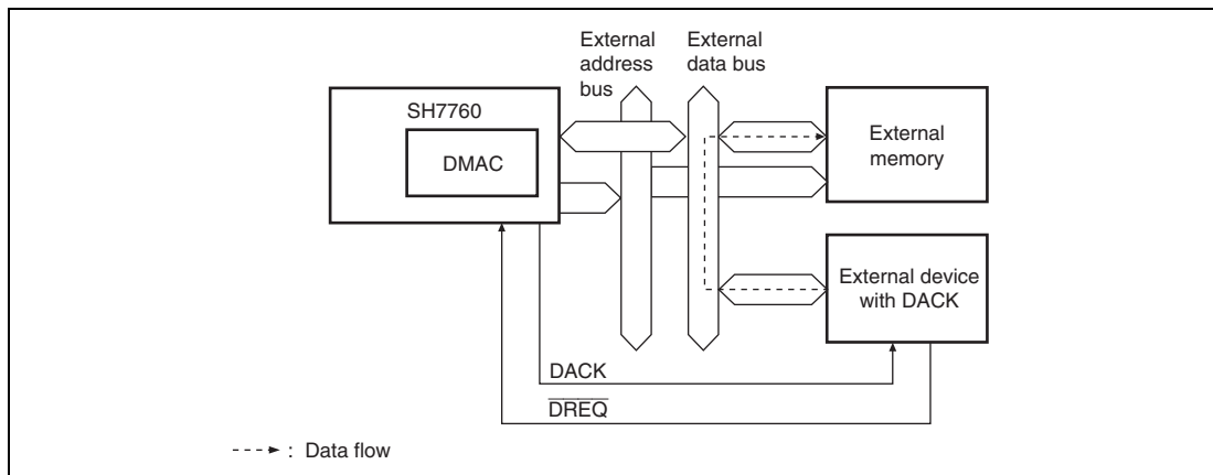
Figure 11.6 Data Flow in Single Address Mode
