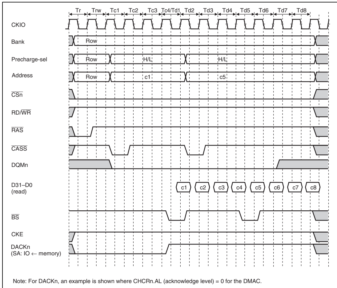
Figure 10.20 Burst Read Timing
