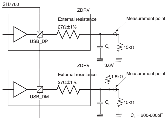
Figure 33.69 Load Condition of AC Characteristics (Low speed)
