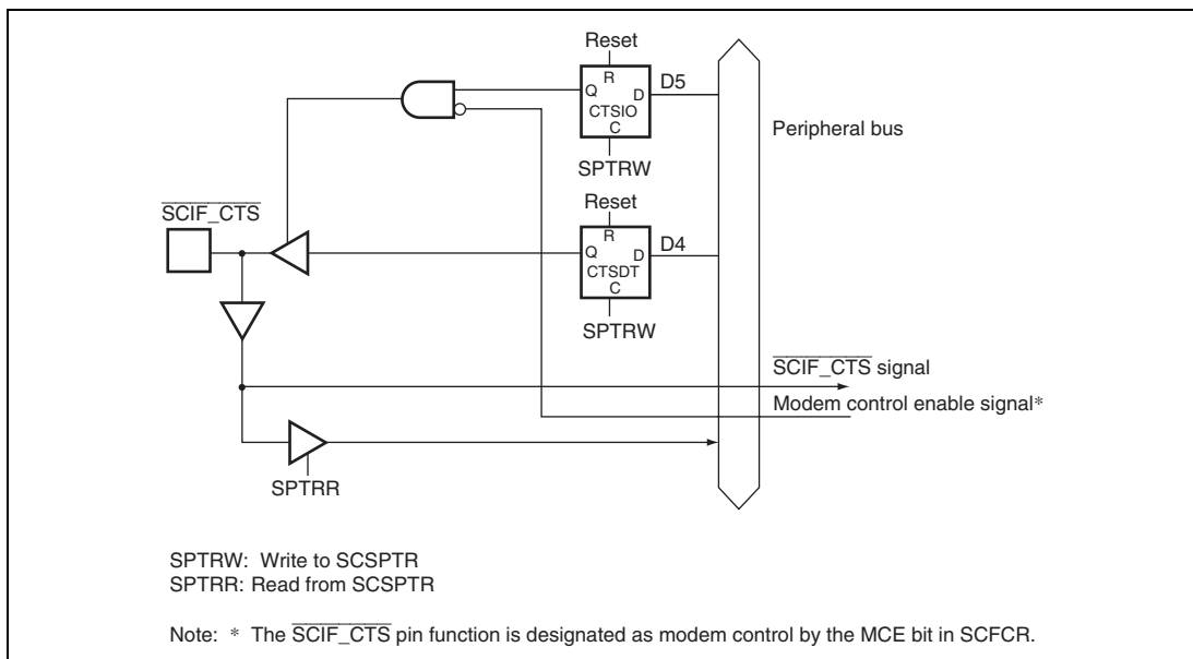
Figure 17.3 SCIF_CT̄S Pin (Only in Channels 1 and 2)
