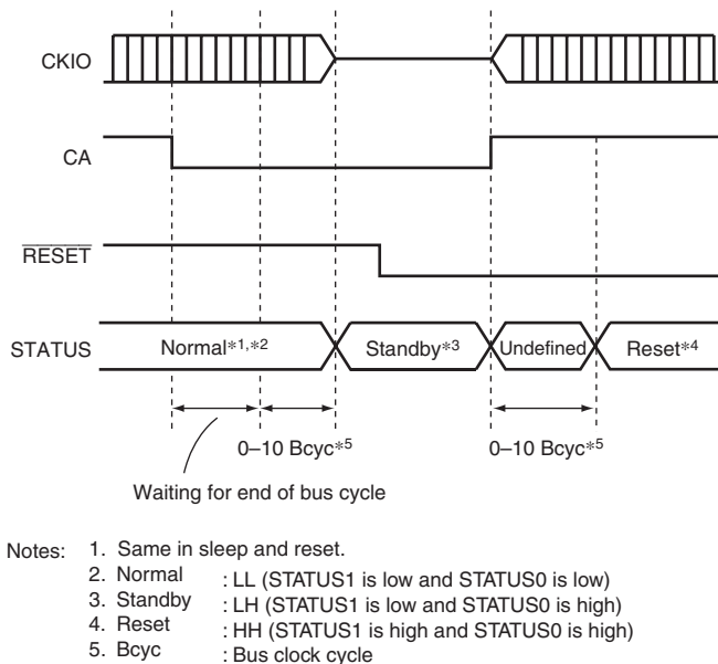
Figure 14.12 Hardware Standby Mode Timing (When CA = Low in Normal Operation)
