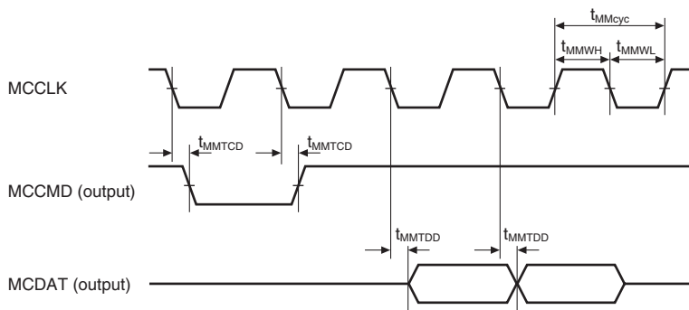
Figure 33.76 MMCIF Transmit Timing
