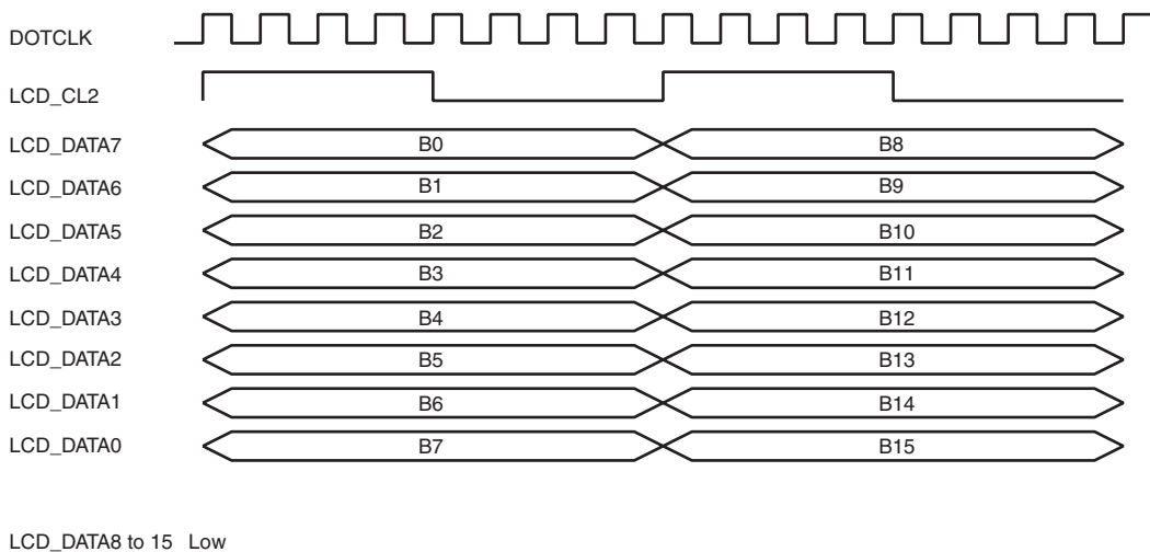
Figure 30.9 Clock and LCD Data Signal Example
