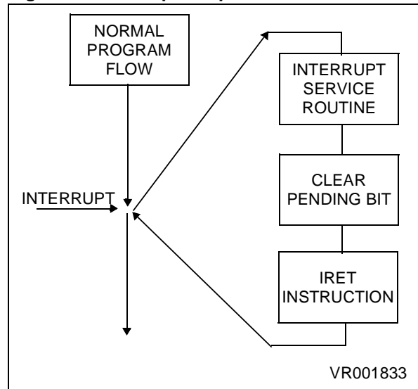
Figure 19. Interrupt Response
