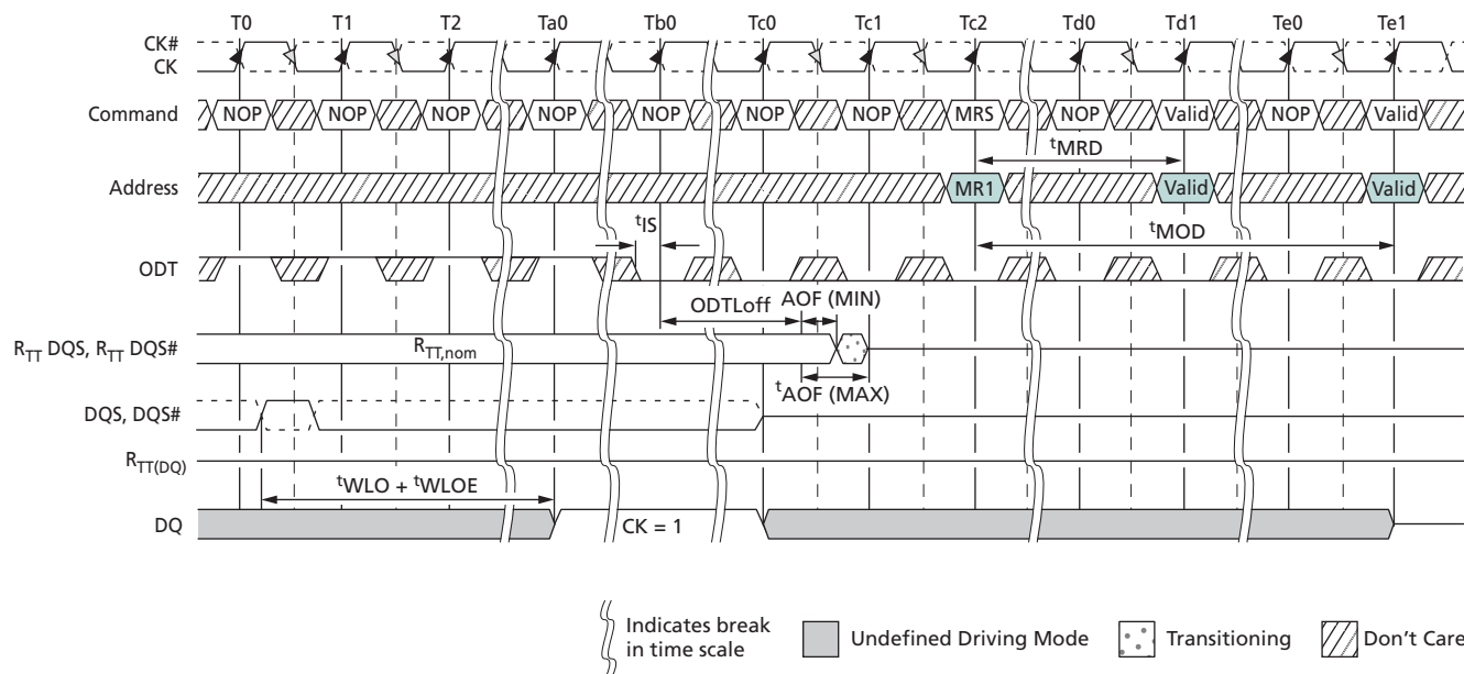
Figure 48: Write Leveling Exit Procedure
