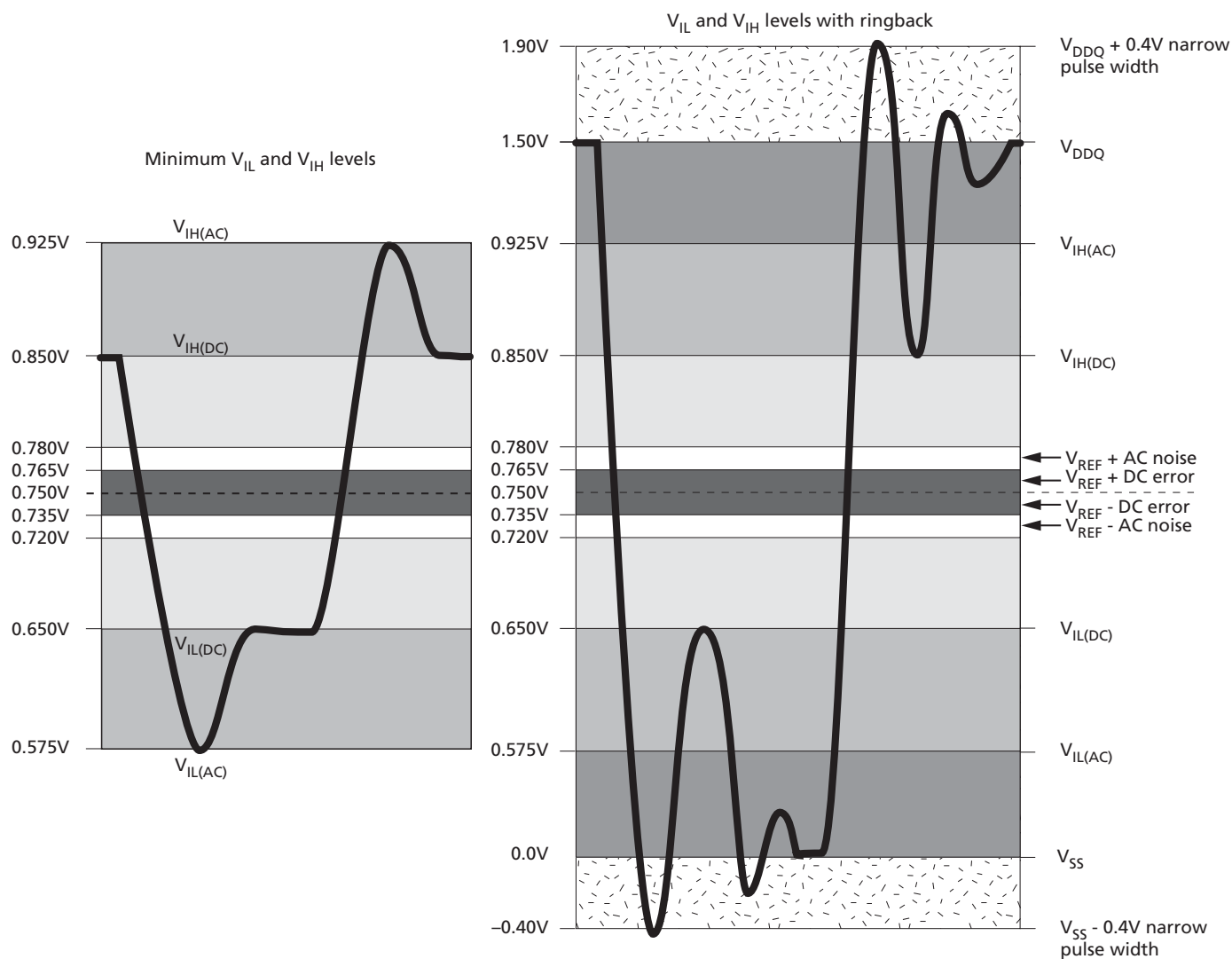
Figure 14: Input Signal
