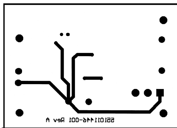
Figure 46. Bottom Layer
