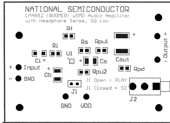
Figure 41. Silk Screen
