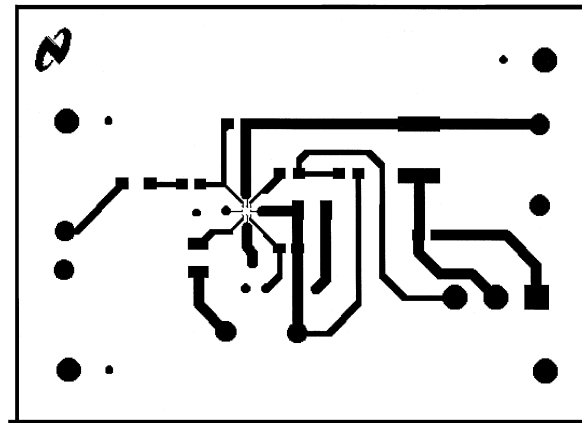
Figure 42. Top Layer
