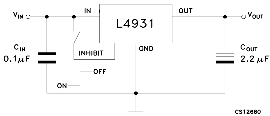
Figure 3. Test circuit
