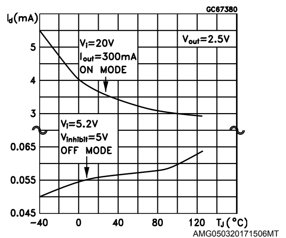
Figure 7. Supply current vs temperature
