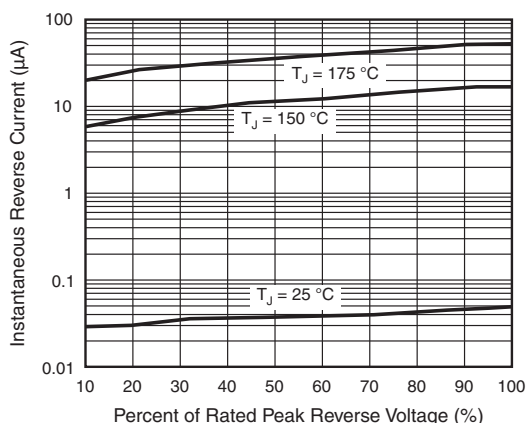
Fig. 4 - Typical Instantaneous Reverse Characteristics
