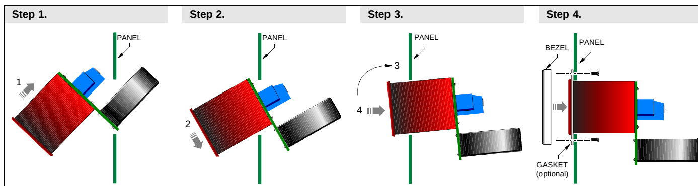
Figure 2. Panel Installation
