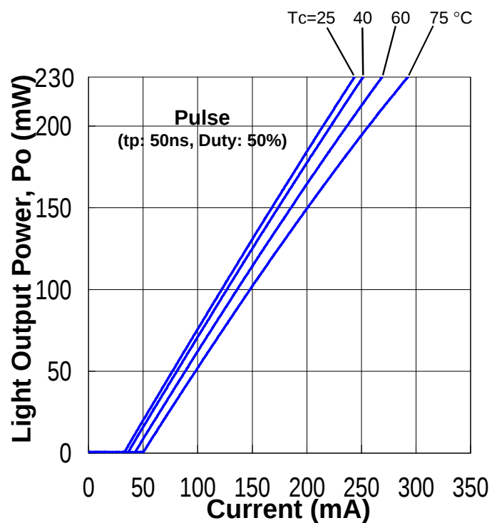
Light Output Power vs. Current (Pulse)
