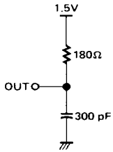
3-STATE TO HIGH
