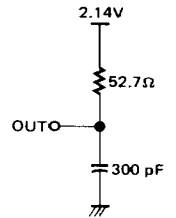
COMMAND OUTPUT TEST LOAD
