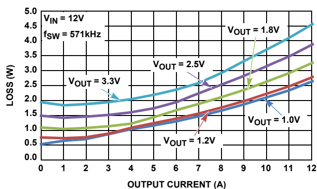
FIGURE 12. POWER LOSS CURVE, 12\text{V}_{\text{IN}} , FOR VARIOUS OUTPUT VOLTAGES LISTED
