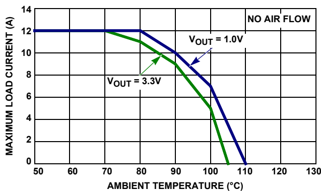
FIGURE 9. DERATING CURVE, 5\text{V}_{\text{IN}} , FOR VARIOUS OUTPUT VOLTAGES LISTED
