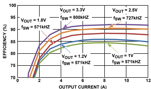
FIGURE 3. EFFICIENCY, V_{\text{IN}} = 9\text{V} , FOR VARIOUS OUTPUT VOLTAGES
