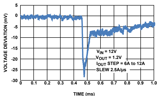
FIGURE 6. DYNAMIC RESPONSE, LOAD
