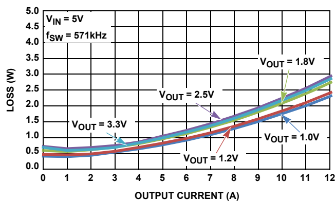
FIGURE 11. POWER LOSS CURVE, 5\text{V}_{\text{IN}} , FOR VARIOUS OUTPUT VOLTAGES LISTED
