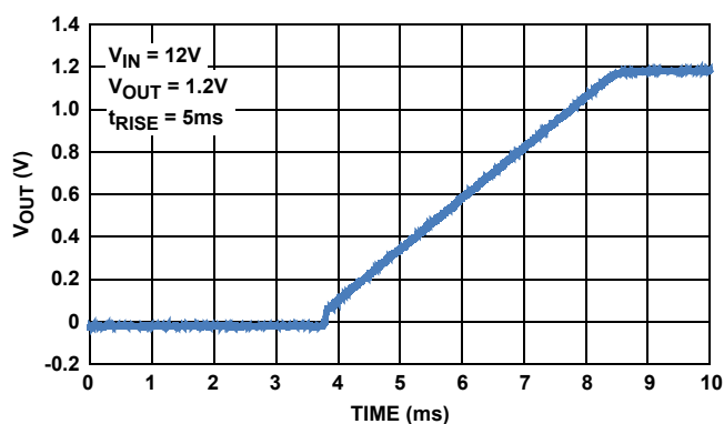
FIGURE 7. SOFT-START RAMP-UP
