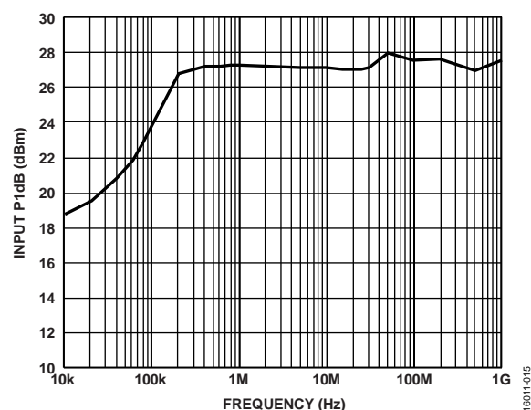
Figure 15. Input P1dB vs. Frequency (Low Frequency Detail)
