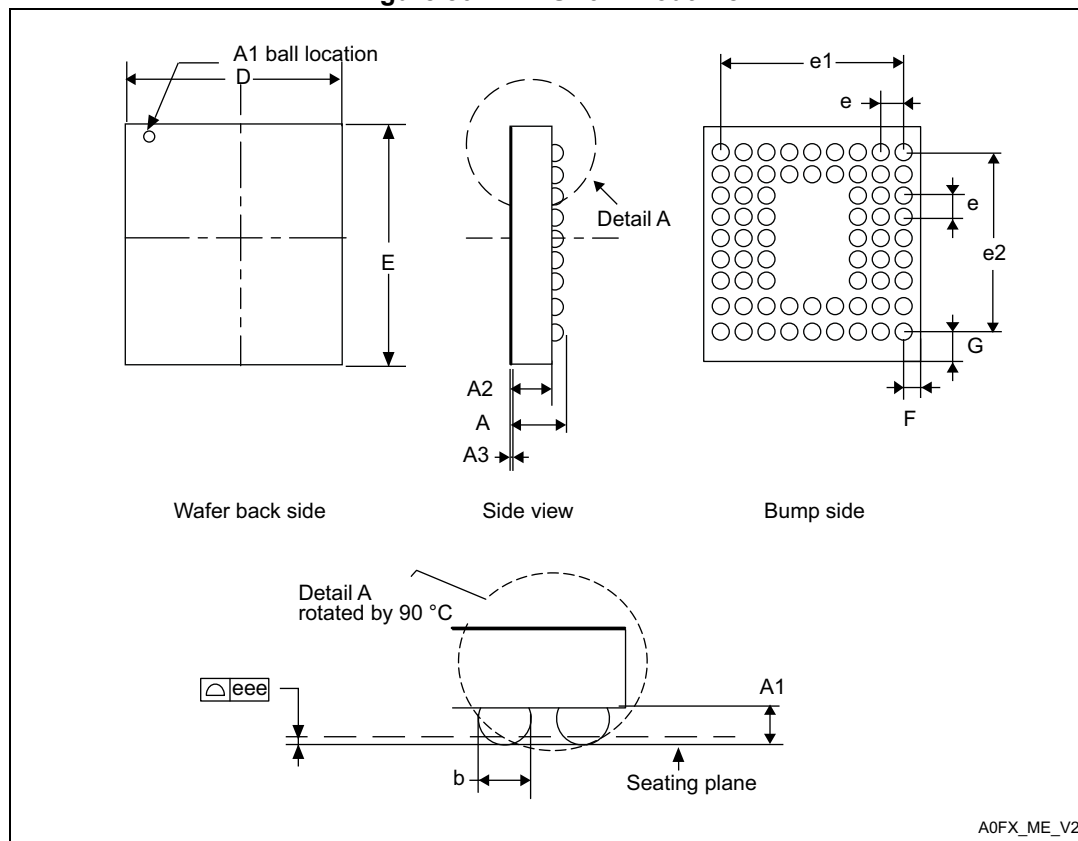
Figure 80. WLCSP64+2 outline
