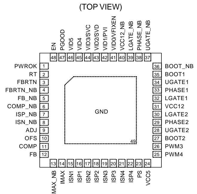
WQFN-48L 7x7
