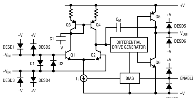
Figure 1. Simplified Schematic
