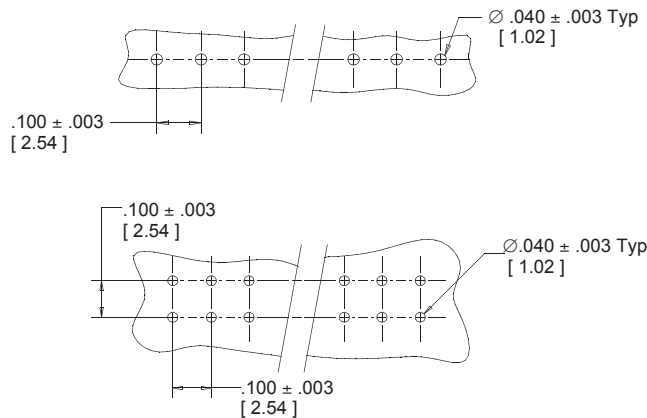
Recommended Mounting Hole Patterns (Shown for Mounting Side of Board)
