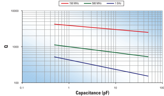
Q vs Capacitance DLI C07 UL Series
