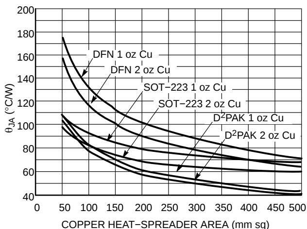
Figure 25. Thermal Resistance
