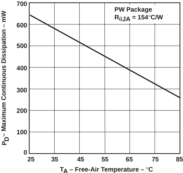
Figure 1. Dissipation vs Free-Air Temperature
