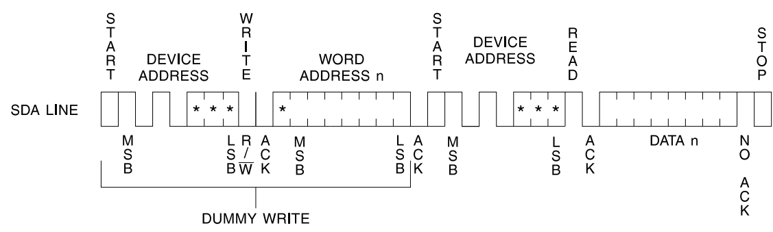
Figure 5. Random Read
