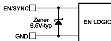
Figure 2: 6.5V-Type Zener Diode
