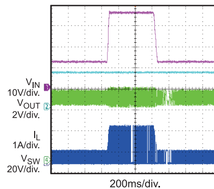
Load Dump
