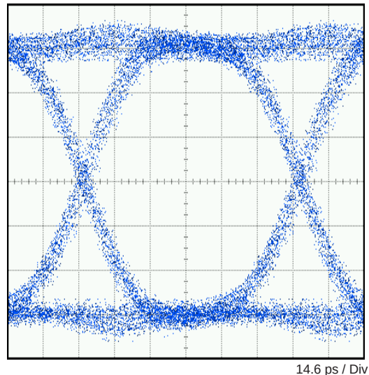
EYE-DIAGRAM AT 11.3GBPS, PRBS-31 PATTERN I_{MOD} = 60\text{ mA} , EQENA = 0
