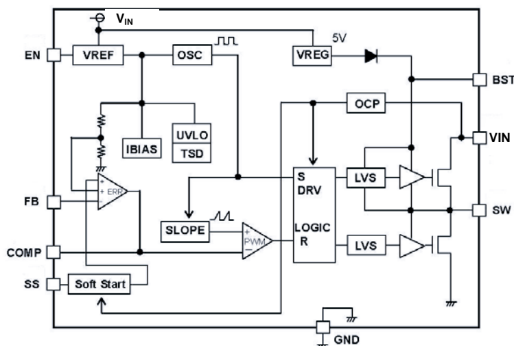
Figure 3. Block Diagram
